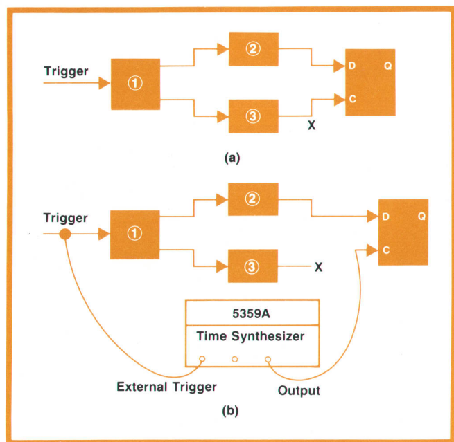
Fig. 1. Model 5359A Time Synthesizer can help test for race conditions in logic systems. In the hypothetical system of (a), an input trigger passes through subsystems 1, 2, and 3 before arriving at the D and C inputs of the flip-flop. Changes in propagation delays through the two paths could result in improper operation of the flip-flop. The problem is to measure the allowable range of delays. The measurement is more difficult if the D input is a data string from which one bit is to be selected, or if the setup time of the flip-flop is unknown. In (b), the time synthesizer output is substituted for the signal at point X. The synthesized delay can be varied easily to determine the limits of proper operation. Because the synthesizer can produce relatively long delays, it can be triggered from the input of the system, which is often easier than finding a suitable internal trigger point.
