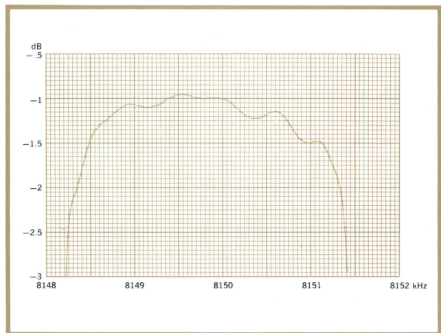
Fig. 3. Passband response of crystal filter shows detail that low residual FM of incremental frequency sweep enables in measurements on narrowband devices. Sweep had 200 frequency steps.
