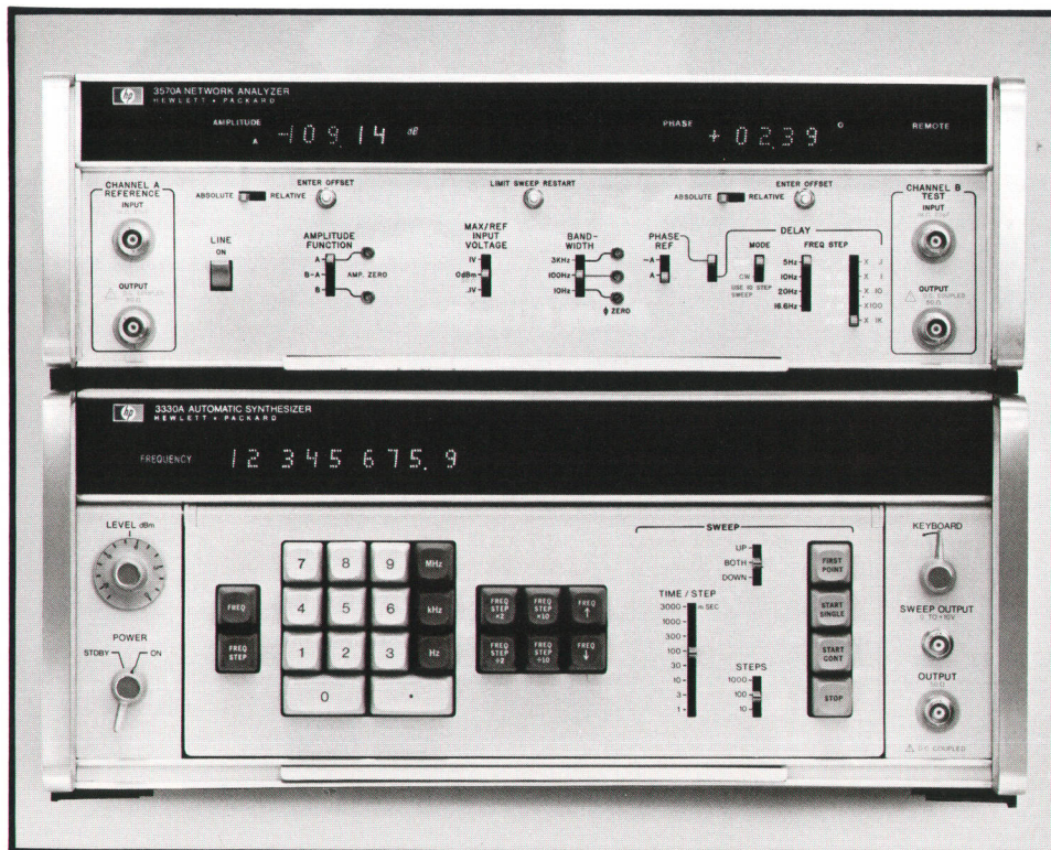
Fig. 1. Model 3570A Network Analyzer (upper unit) functions as two-channel tracking detector with one of HP's 0-13 MHz Frequency Synthesizers (lower unit) to form complete network analysis system. Network Analyzer shown here has Delay / Limit Test / Offset option.
