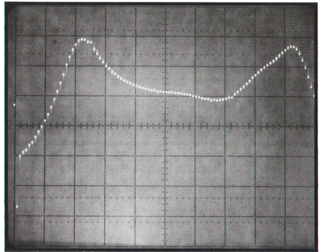
Fig. 2. Group delay vs frequency of FM IF filter as measured by Network Analyzer equipped with Delay/Limit Test/Offset option. Center frequency is 10.7 MHz, horizontal scale is 50 kHz/div, vertical scale is 1 \mu s/div.
