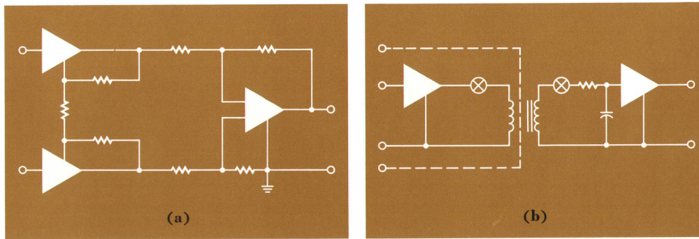
Fig. 1. Two common configurations of data amplifiers are the direct-coupled differential (a) and the carrier-coupled design (b).
