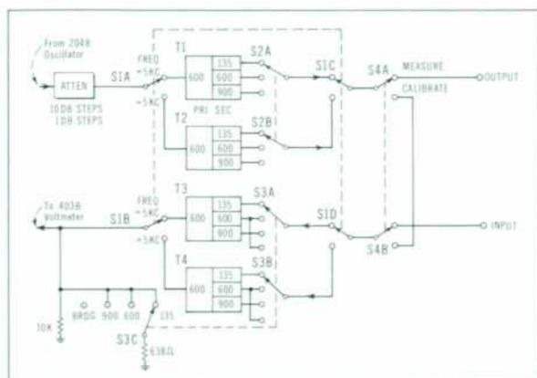
Fig. 3 (at left). Skeleton schematic of patch panel in new test set.
