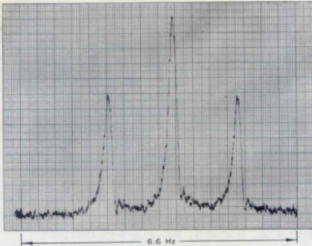
Typical plot obtained by the modulation method. Sample is CF_3CF_2COOH .
