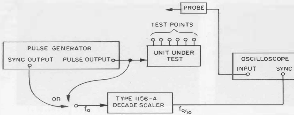
Figure 4. Oscilloscope synchronizing setup for testing decade scalars and frequency dividers.
