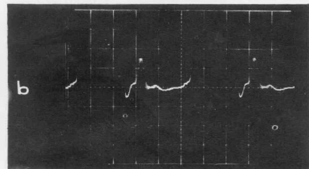
Figure 10. Resolution of pulse pairs when first pulse has 10 times the amplitude and 4 times the duration of the second pulse. For (a), upper trace shows input, lower trace output; vertical, 1 V/cm; horizontal, 50 ns/cm. (b), input signal expanded to show smaller pulse; vertical scale is 0.1 V/cm; horizontal, 10 ns/cm.
