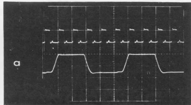
Figure 8. Operation on brief pulses at 105 Mc/s. Positive pulses at left, negative at right. Upper trace shows input; vertical scale is 0.1 V/cm. Lower trace shows output into 50 ohms; vertical scale is 0.5 V/cm. For (a), horizontal scale is 10 ns/cm; for (b), 2 ns/cm.
