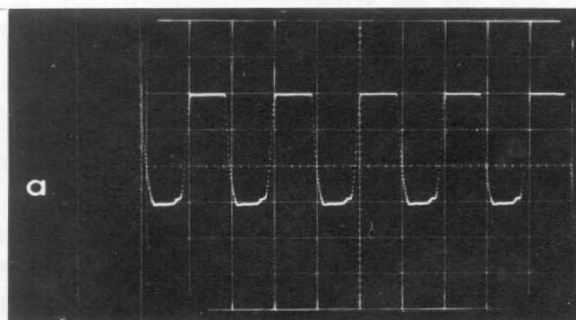
Figure 3. Output into 50 ohms. (a) 5 Mc/s (50-Mc input); (b) 12.5 Mc/s (125-Mc input). Vertical scale is 0.5 V/cm.
