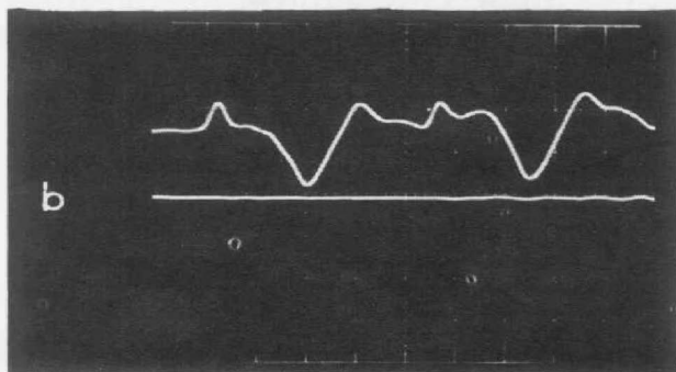
Figure 9. Resolution of pulse pairs occurring at a 20-Mc rate. Upper trace shows input; vertical scale is 0.1 V/cm. Lower trace shows 4-Mc output into 50 ohms; vertical scale is 0.5 V/cm. For (a), horizontal scale is 50 ns/cm, for (b), 2 ns/cm.
