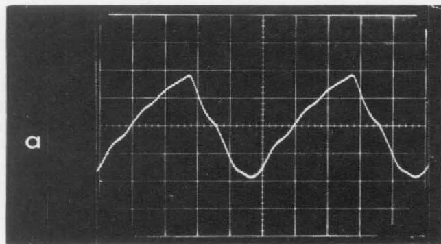
Figure 2. Scaler output waveforms (a) 10 Mc/s (100-Mc input); (b) 12.5 Mc/s (125-Mc input). Vertical scale is 1 V/cm. Measurement setup is shown at right.
