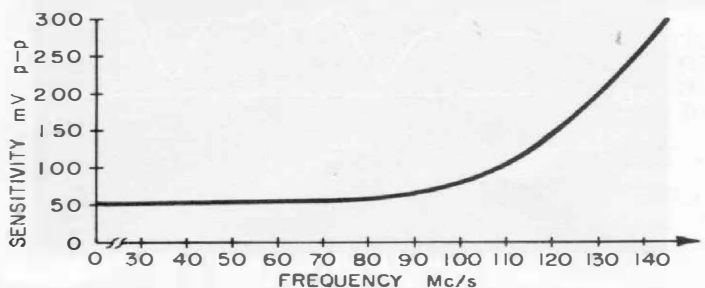
Figure 7. Scaler sensitivity vs frequency. The scaler will operate reliably over a temperature range of 0 to 50°C with an input frequency of at least 125 Mc/s and a sensitivity of better than 300 mV, peak-to-peak.
