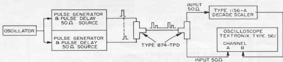
Figure 12. Test setup for Figure 10.
