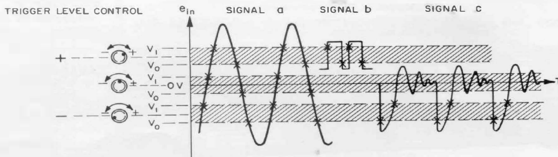
Figure 2. The trigger-level control adjusts the input trigger point. The control settings and the corresponding trigger points are shown for three types of input signals.
