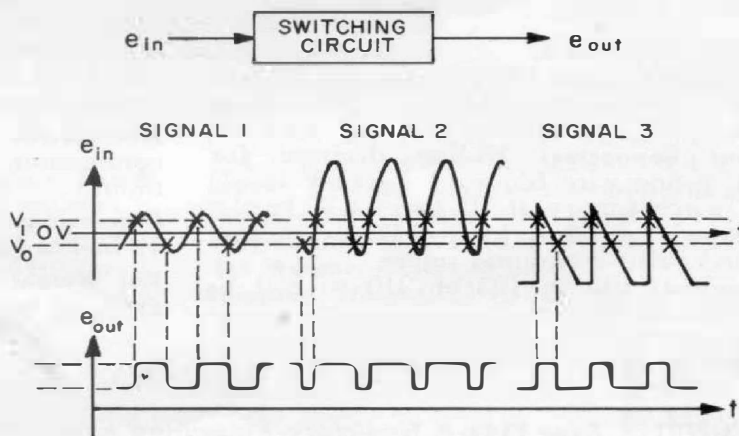
Figure 1. Switching-circuit input trigger points and corresponding output signals for three different input signals.
