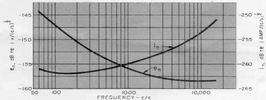
Figure 2. Typical frequency spectra of internal noise.
