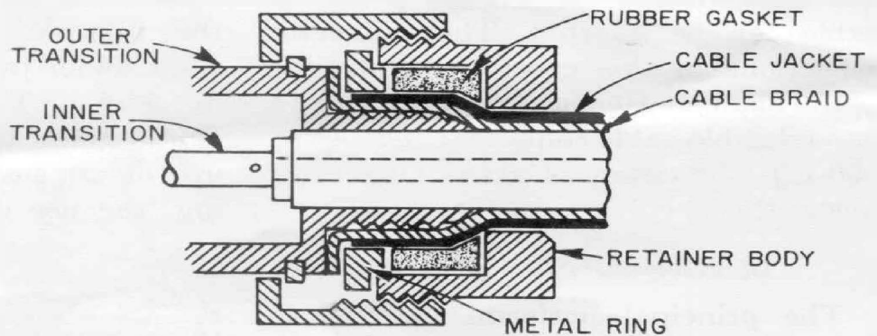
Figure 2. Braid and jacket-retention system shown before coupling ring is tightened.
