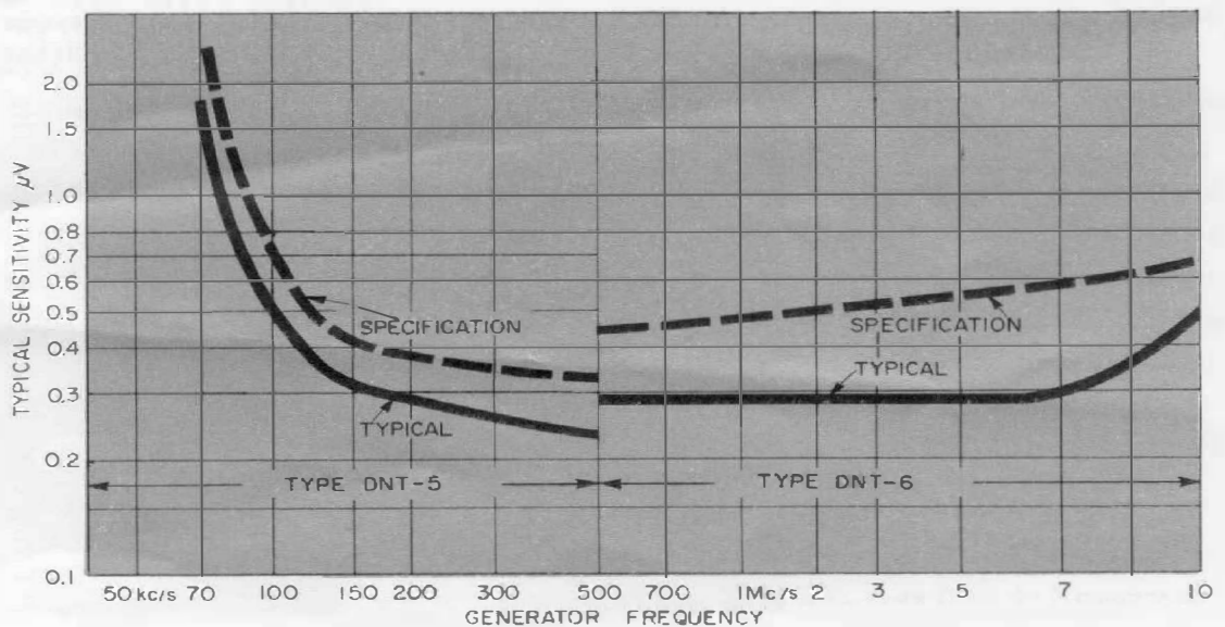
Sensitivity vs frequency for Type DNT-5 and Type DNT-6 Heterodyne Detector.
