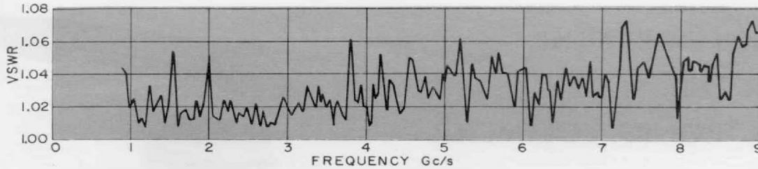
Figure 3. Typical VSWR of a single Type 900-C9 Connector on "infinite" length of RG-214/4 cable.
