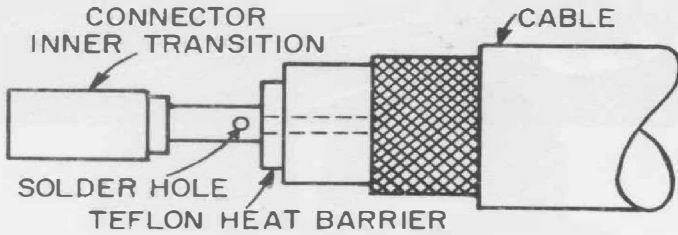
Figure 1. Inner-transition assembly showing Teflon disk.
