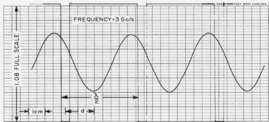
Figure 5. Multiple recording used in direct measurement of VSWR and phase.
