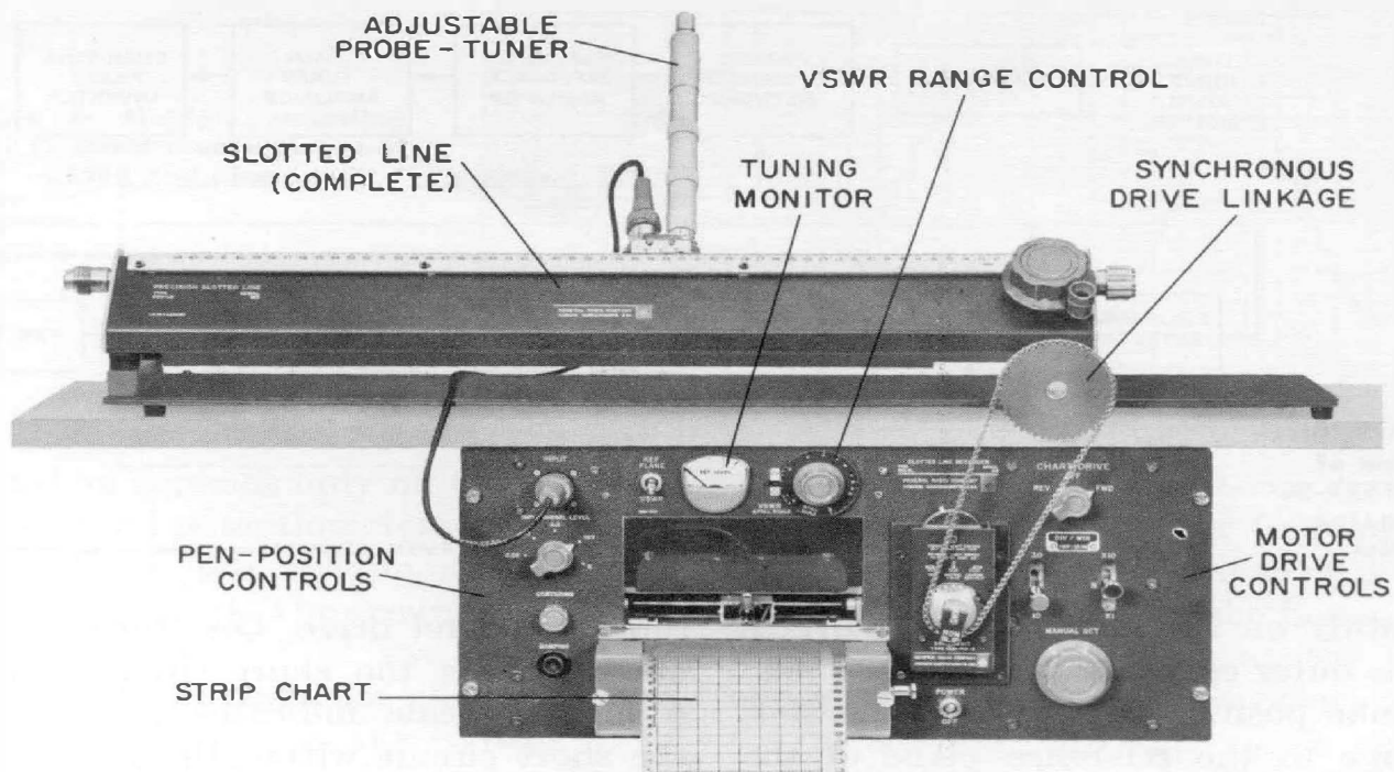
Figure 2. Type 1640-A Slotted Line Recorder System. Owners of Type 900-LB Slotted Lines can easily add recorder and connecting linkage. Prices are available on request.
