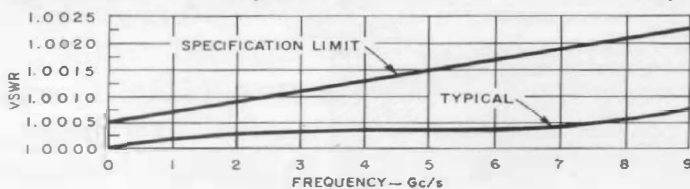
Figure 4. VSWR characteristics.
