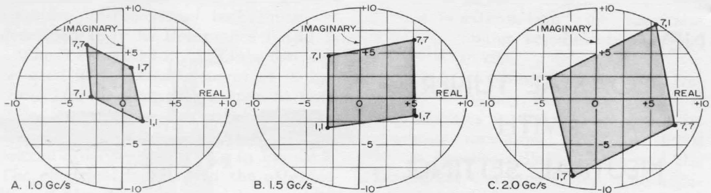
Figure 3. Smith-chart plots showing tuning range of Type 900-TUA Tuner. Numbers at corners are settings of screws 2 and 3, respectively. Tuning screw 1 is set at 5.00. Axis values are in terms of percent deviation from match. A 10-percent mismatch corresponds to a VSWR of 1.100.
