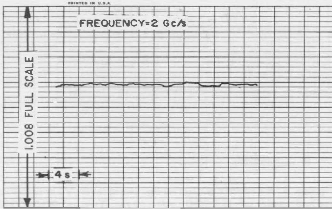
Figure 10. Typical recording of system noise at 2 Gc/s, with Type 1360-B Microwave Oscillator used as signal source. Chart speed was 30 div/min. Note that total excursion over entire 25-second recording is equivalent to VSWR of only 1.0002.
