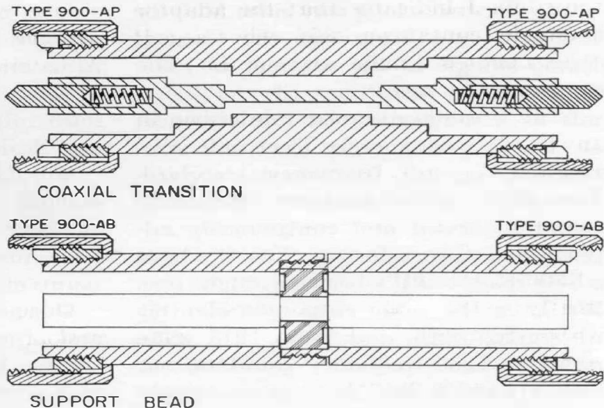
Figure 1. Cross-section view of coaxial line sections fitted with Types 900-AP (top) and 900-AB Precision Coaxial Connector Kits. Type 900-AP connection is same as that used in the Type 900-LZ Reference Air Lines.
