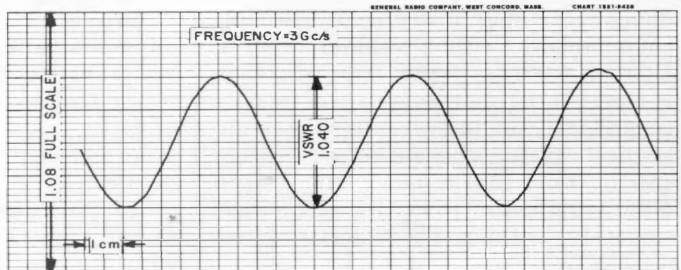
Figure 4. Typical direct recording of vswr .
