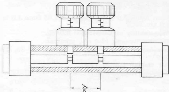
Figure 2. Cross-section view of tuner.
