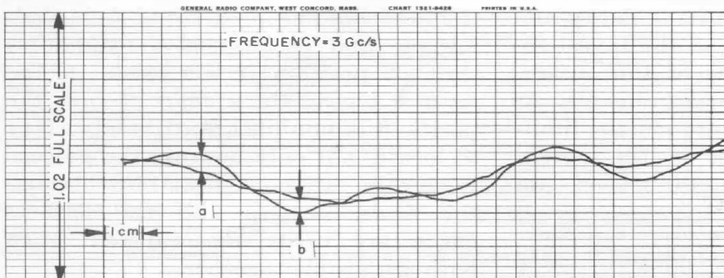
Figure 1. Multiple plot used to measure difference between two measurement conditions. Note that the difference in the recording ( a + b ) is a sine wave corresponding to a VSWR of 1.002!
