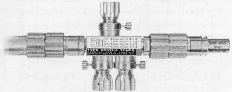
Figure 1. Type 900-TUA Tuner, shown in place between reference air line and Type 900-W50 50-ohm Standard Termination.
