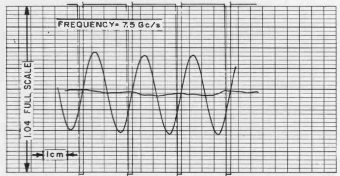
Figure 8. Recording showing insertion VSWR of a mated pair of GR900 adaptors (Types 900-QNJ and -QNP) at 7.5 Gc/s.
