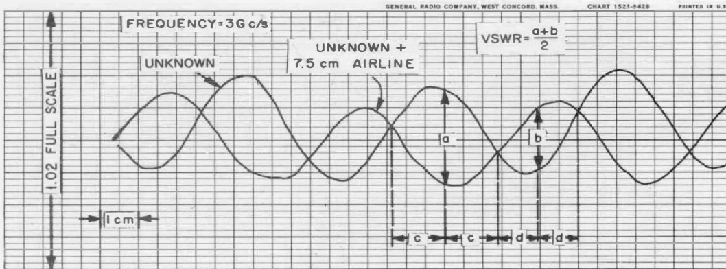
Figure 6. Multiple recording used in substitution - method VSWR measurement.
