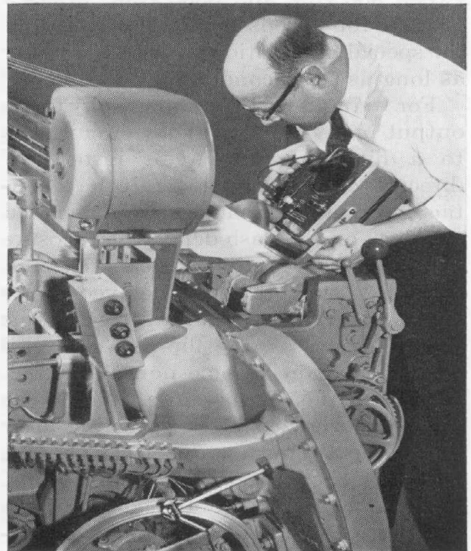
Figure 5. A typical application in the textile field: observing tape and filling-carrier behavior of a Draper DSL shuttleless loom. Speed of the filling carrier is 274 picks per minute. The Flash Delay makes it possible to observe the filling-carrier at any particular point on its path. Synchronism with loom is accomplished with the Type 1536-A Photoelectric Pickoff located near a rim connected to the main power shaft and shown at the bottom of the photograph.
