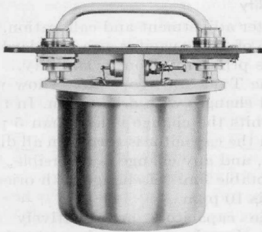
Figure 4. View of capacitor with cabinet removed, showing the sealed container and the three-terminal trimmer.
