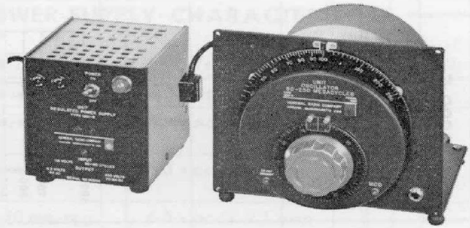
Figure 5. Oscillator with older type of Unit Power Supply, Type 1201-B.
