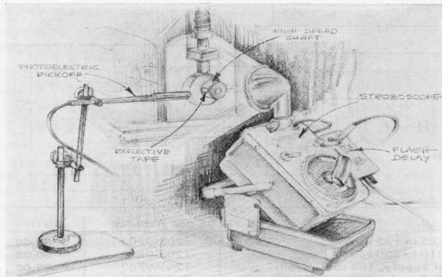
Figure 2. Sketch showing the use of reflective tape to produce a pulse signal in the Photoelectric Pickoff. Pulse is then delayed by the Flash Delay to fire the Strobotac at any desired point in the rotational cycle.
