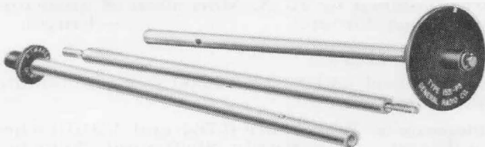
Figure 1. View of the Surface-Speed Wheel, showing the two speed discs and the sectional shaft.
