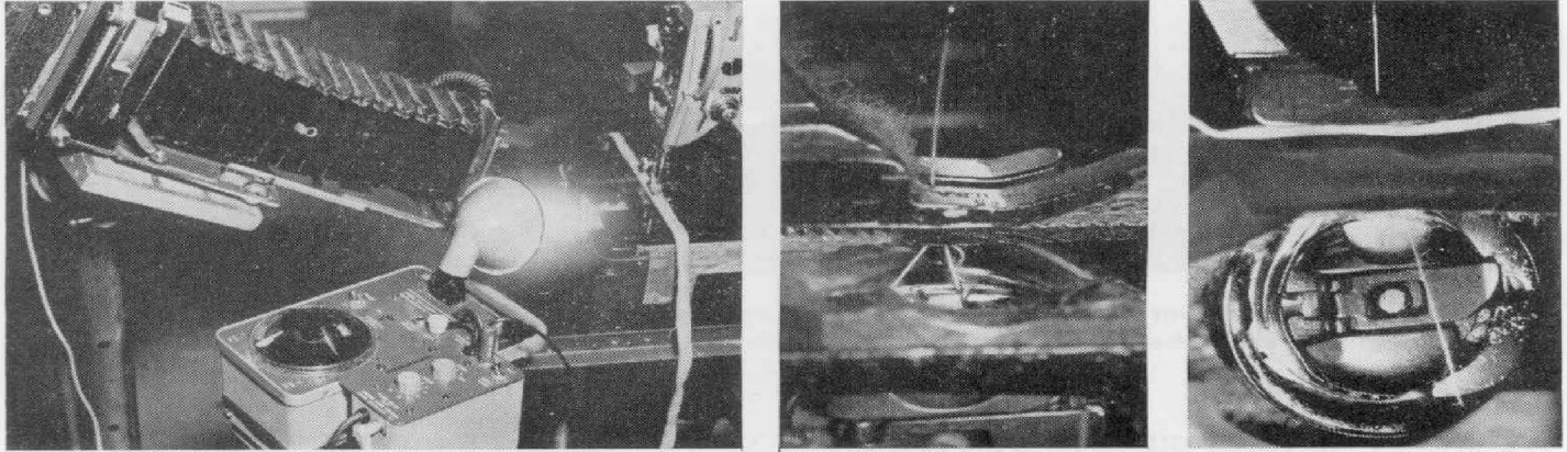
Figure 6. Study of thread behavior in high-speed sewing machine. Machine speed was 5000 stitches per minute; hook speed was 10,000 rpm. Photograph at left shows setup using Linhoff 4 x 5 with Polaroid film, Strobotac with attached Flash Delay, and sewing machine (the base of which is cut away to expose the parts underneath). Center and right photographs show the bobbin and hook action on thread at a specific phase selected by means of the Flash Delay. Photographs courtesy of The Singer Company.
