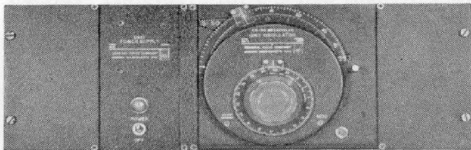
Rack-mount arrangements of a Unit Oscillator with two types of power supply. Figure 3 (left) shows the Type 1269-A Power Supply; Figure 4 (right) the Type 1263-B Amplitude-Regulating Power Supply. For bench mount, the rack-adaptor plates, shown at the ends of the assemblies, are not used.
