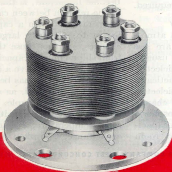
Figure 1. View of the 1000-pf capacitor removed from its cabinet and sealed container, showing the construction of the plate stack.
