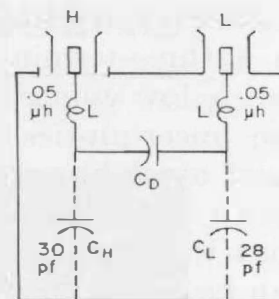
Figure 5. Equivalent circuit of Type 1404 Capacitors. C_D = 1000 pf for Type 1404-A C_D = 100 pf for Type 1404-B
