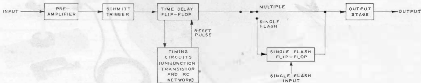
Figure 3. Functional block diagram of the Flash Delay.
