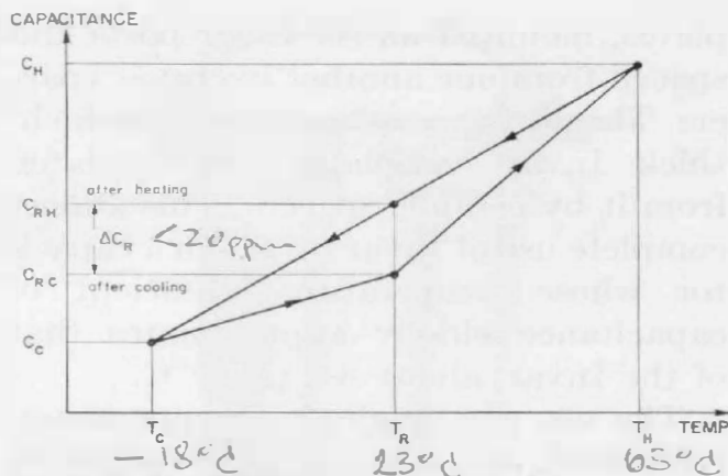
Figure 2. Capacitance vs temperature diagram showing hysteresis.
