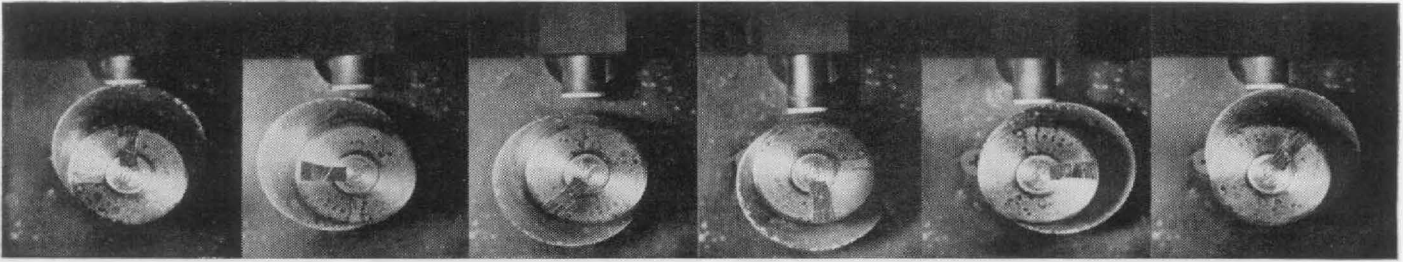
Figure 4. The action of cam followers can be easily examined with the Strobotac-Flash Delay combination. These photographs show the bounce of a cam follower at high speeds. The cam is rotating counterclockwise.
