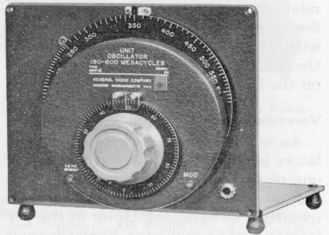
Figure 1. Panel view of the Type 1209-CL Unit Oscillator.
