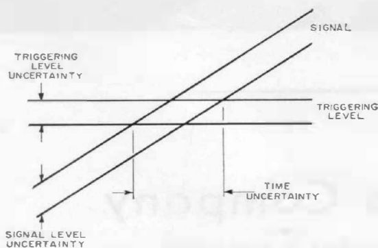
Figure 8. Effects of uncertainty in signal or triggering level.
