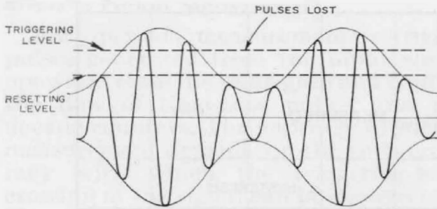
Figure 5. Error caused by amplitude modulation.
