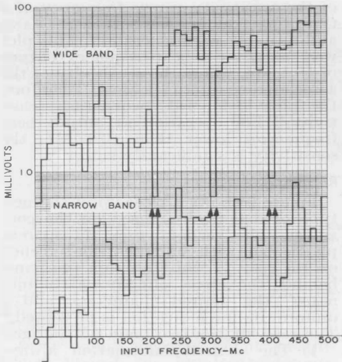
Figure 5. Typical over-all sensitivity of converter and counter for 10.1-Mc counter indication. This is worst case. Sensitivity is better for lower converter output frequencies.
