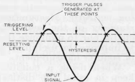
Figure 4. Operation of input circuits.
