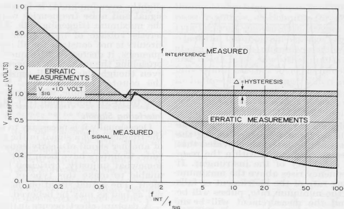
Figure 7. Capture behavior of a counter. Counter ignores an interfering signal with amplitude below the shaded area. If interference amplitude exceeds shaded area, counter will measure interfering signal only.
