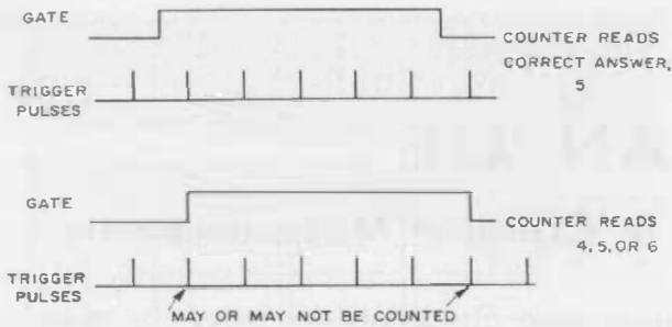
Figure 2. One-count gating error. Pulses occurring simultaneously with the gate may or may not be counted.
