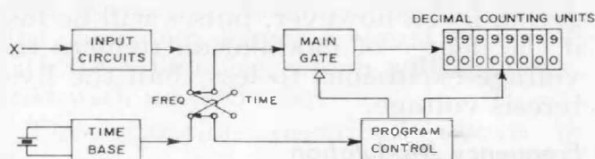
Figure 1. Simplified block diagram of a digital time and frequency meter.
