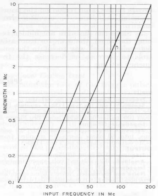
Figure 4. Tuned-amplifier bandwidth versus frequency. For input frequencies above 200 Mc, amplifier operates from 10 to 100 Mc.
