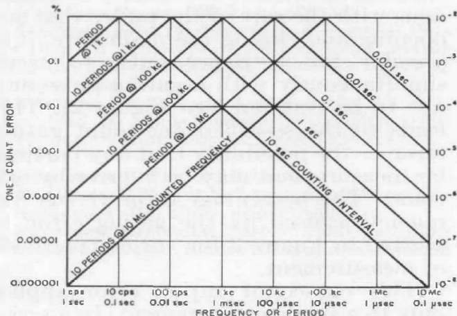
Figure 3. Percentage error versus frequency caused by one-count gating error.
