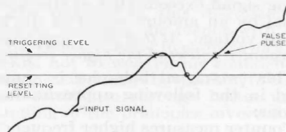
Figure 6. Effects of additive noise.
