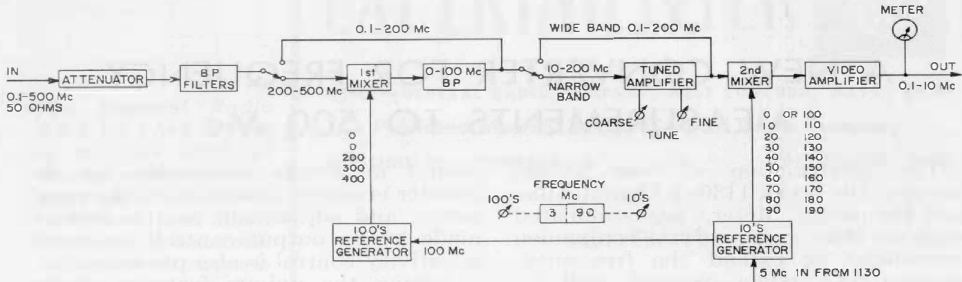
Figure 2. Over-all block diagram. A single conversion system is used below 200 Mc, a double conversion system from 200 to 500 Mc.
