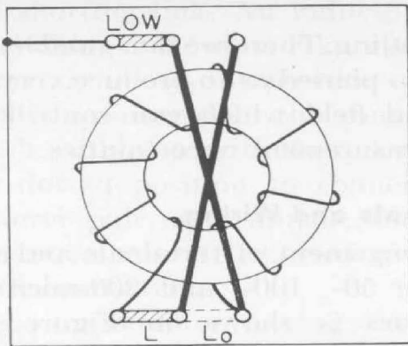
Figure 2. New six-terminal panel and connections.
