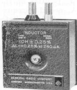
(Left) Type 1481-N Inductor; (center) Type 940-DD Decade-Inductor Unit; (right) Type 1490-F Decade Inductor.
