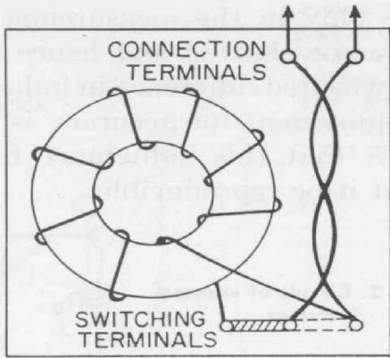
Figure 4. Inductor with shunting link arranged to disconnect coil when short is connected.
