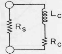
Figure 3. Circuit of shorted inductor.
