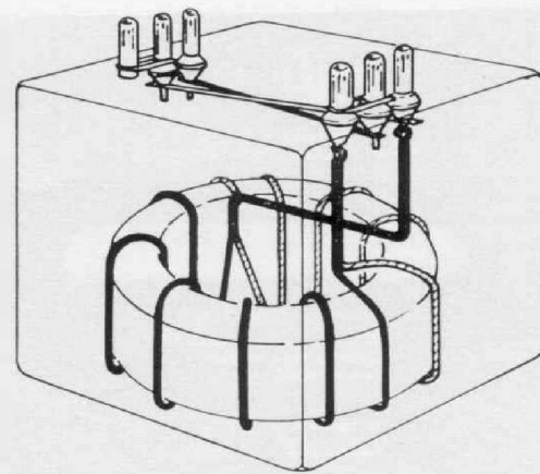
Figure 1. Diagram of duplex winding used for low-inductance standards.
