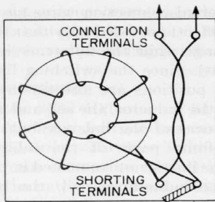
Figure 2. Inductor with separate terminals for connection and for shorting.
