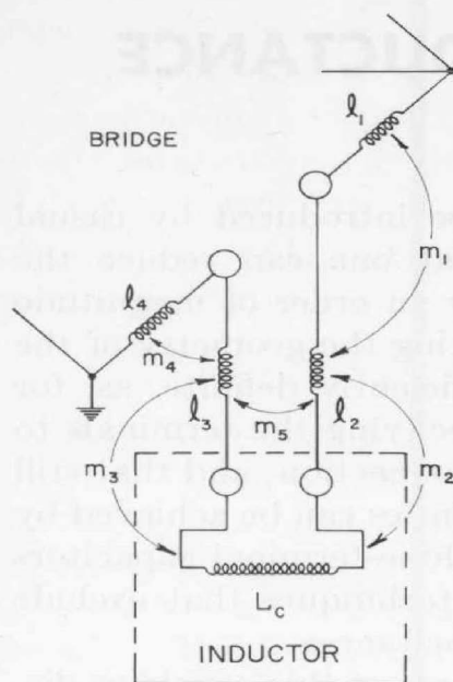
Figure 1. The circuit of an inductor connected to a bridge showing self and mutual inductances which are measured.
