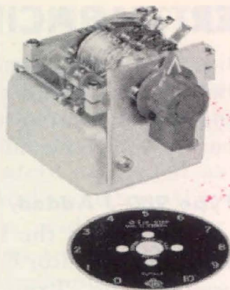
(Left) Type 1419 Decade Capacitor; (right) Type 980-L Decade-Capacitor Unit.
