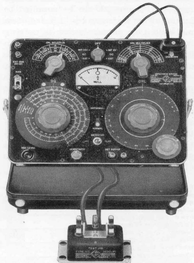
Figure 9. Bridge with Test Jig connected.
