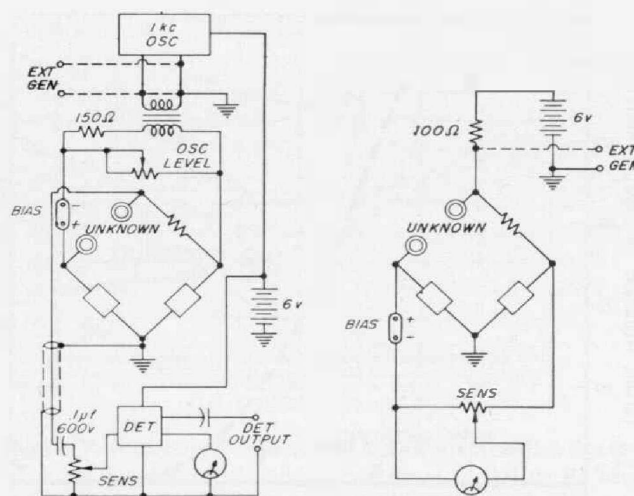
Figure 3. Block schematic of the bridge generator and detector. External-generator connections are shown by dashed lines.
