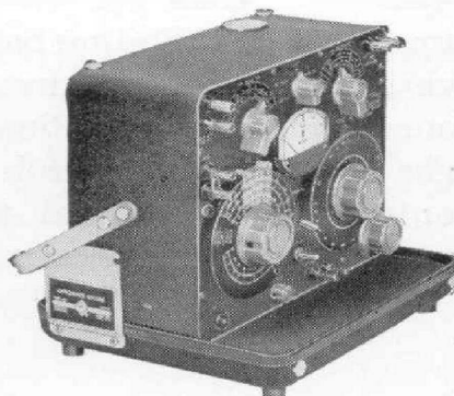
Figure 5a (Left). Bridge cabinet when closed is an easily carried, protective case. Figure 5b (Center). Bridge, when cabinet is opened, can be used with panel vertical or, as shown in Figure 5c (right), tilted at any desired angle.
