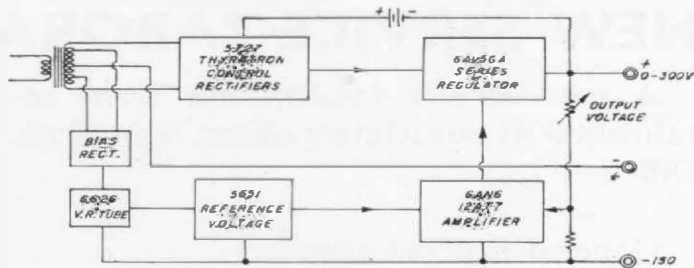
Figure 2. Block schematic of the power supply.
