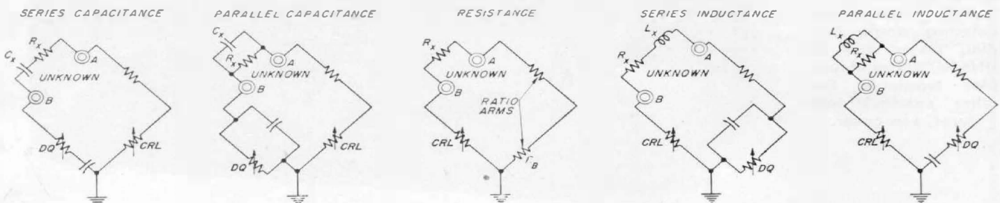
Figure 2. The five circuits used in the bridge.
