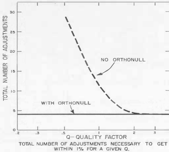
Figure 4. Plot of total number of balances required to achieve final balance, with and without Orthonull , as a function of Q .
