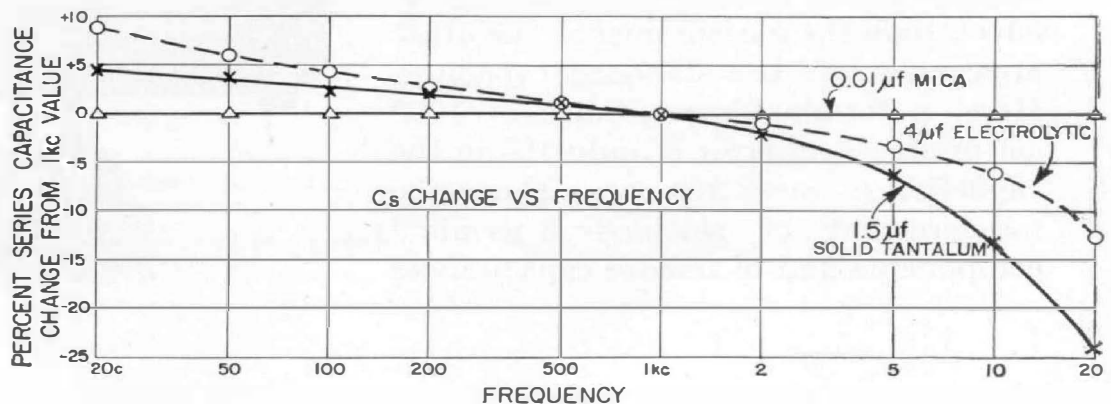
Figure 6. Plots of capacitance vs. frequency for three types of capacitors, as measured on the Type 1650-A Impedance Bridge. The 1210-C Unit R-C Oscillator was the external, variable-frequency generator.
