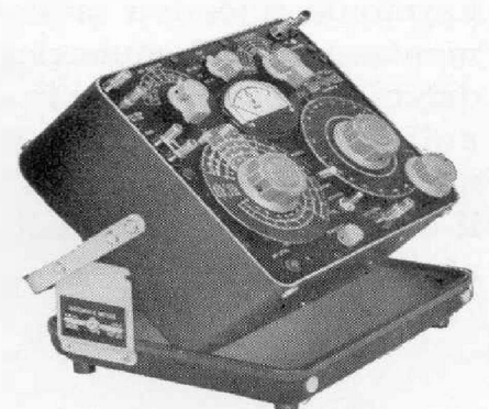
Figure 5a (Left). Bridge cabinet when closed is an easily carried, protective case. Figure 5b (Center). Bridge, when cabinet is opened, can be used with panel vertical or, as shown in Figure 5c (right), tilted at any desired angle.
