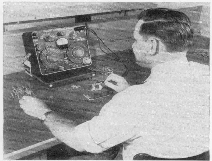
Figure 10. With the Test Jig, as shown here, the bridge can be set up for go-no-go testing to preset limits.
