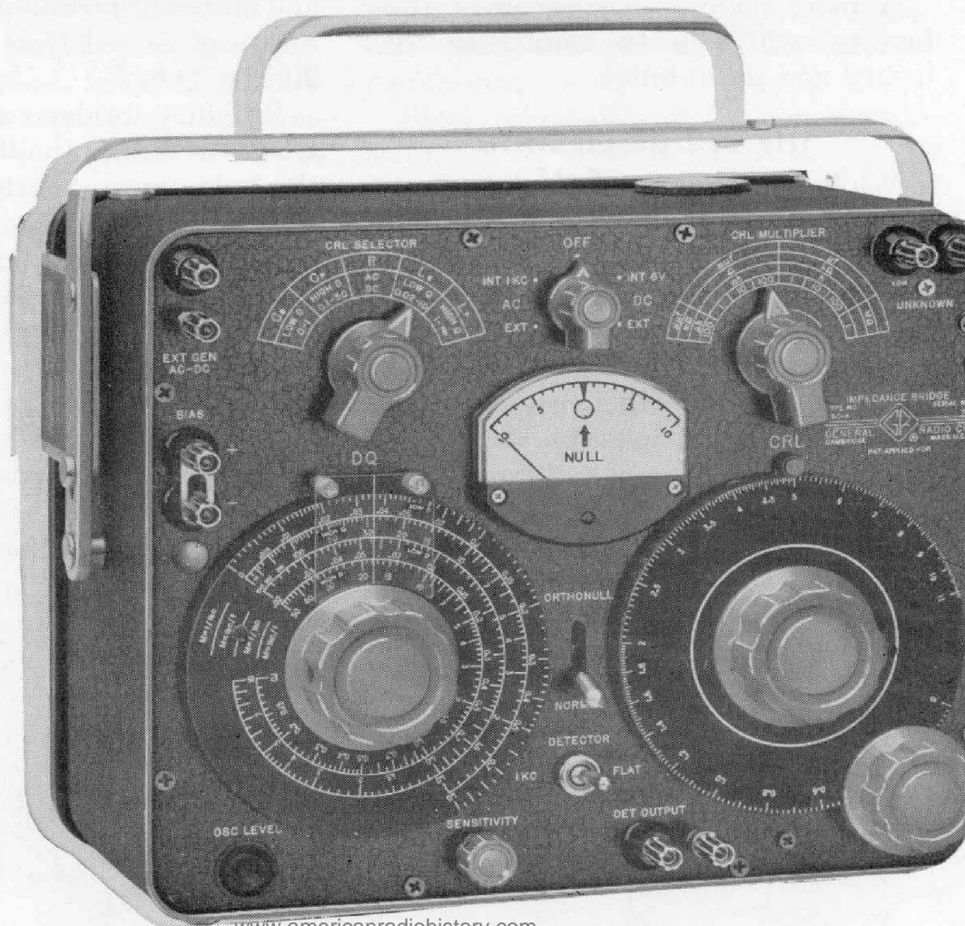
Figure 1. Panel view of the Type 1650-A Impedance Bridge. Note the many new features: Orthonull; built-in generator and detector; single D - Q dial; single pair of UNKNOWN terminals; bias terminals. For other external features, see cover.
