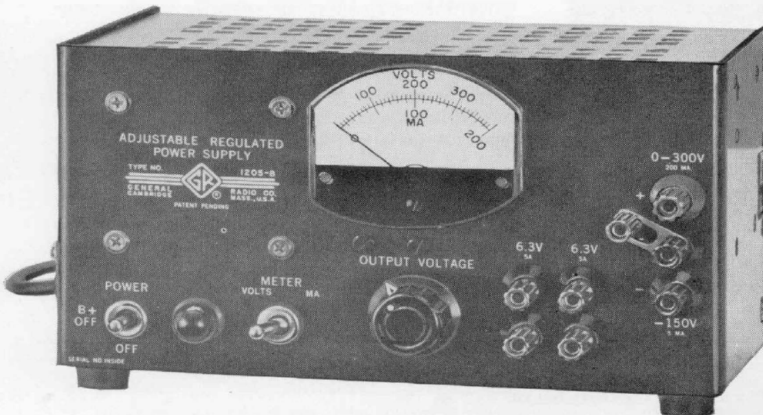
Figure 1. Panel view of the Adjustable Regulated Power Supply.
