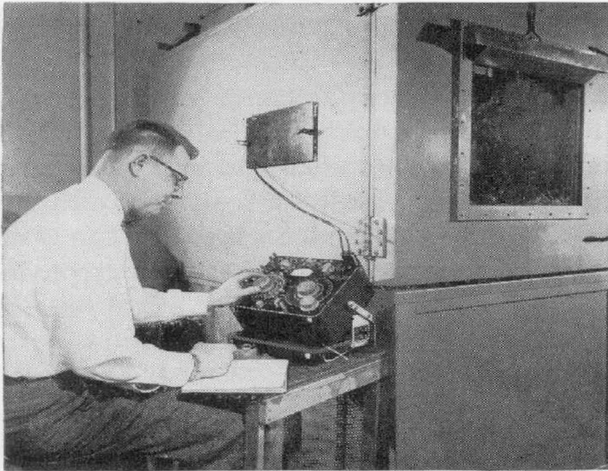
Figure 11. Bridge in use for 3-terminal measurements of sample in conditioning chamber.
