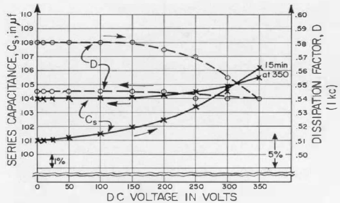
Figure 7. Measured capacitance and dissipation factor of a new electrolytic capacitor as a function of impressed dc voltage as it is passed to its rated voltage, then returned to zero bias.
