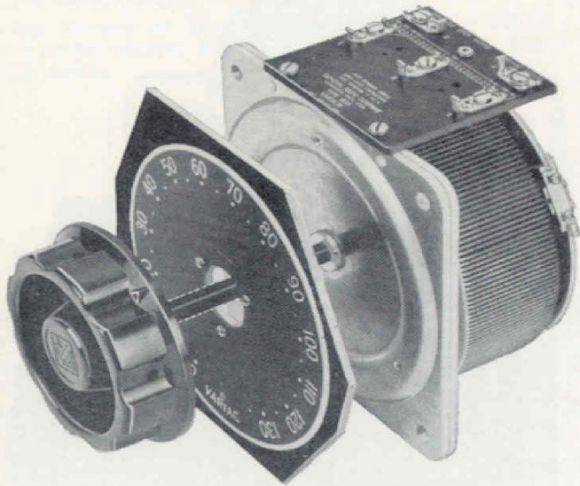
Figure 1. Uncased, 115-volt model, Type W20.
