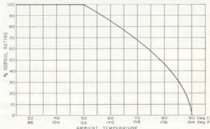
Figure 6. For ambient temperatures above 50°C., Variacs should be derated according to this curve.
