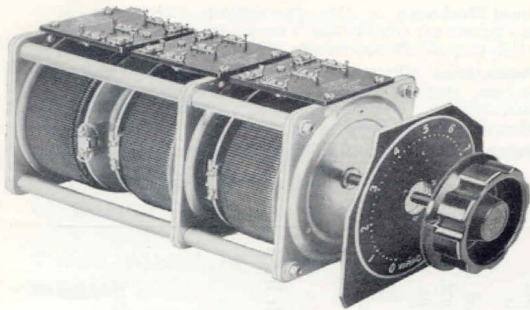
Figure 4. Uncased three-gang assembly, Type W20G3.
