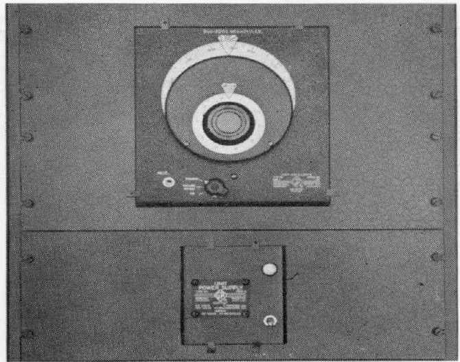
Figure 2. View of the Type 1218-A Unit Oscillator and the Type 1205-A Unit Power Supply mounted in the Type 480-P7U1 and the Type 480-P4U1 Relay-Rack Panels, respectively.
