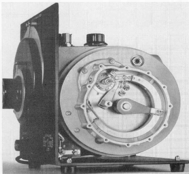
Figure 4. View of the right-hand end of the oscillator assembly with cover removed to show the cathode line.
