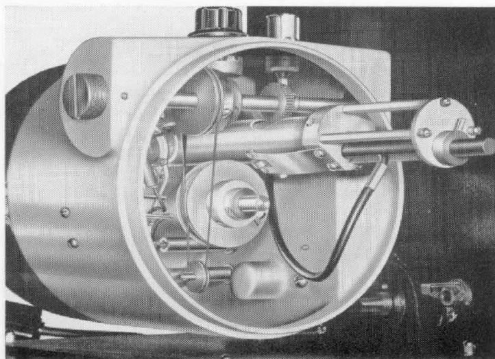
Figure 5. View of the left-hand end of the oscillator casting with cover removed showing the drive mechanism.
