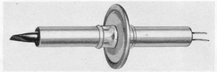
Figure 3. The 5675-type pencil tube used in the Type 1218-A Unit Oscillator.
