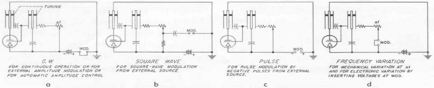
Figure 6. Schematic diagrams of oscillator for various modulation conditions.
