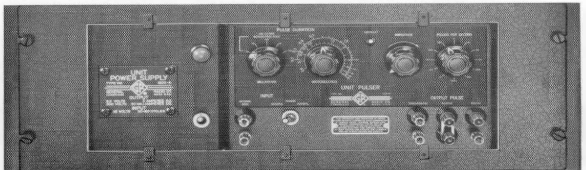
Figure 1. View of the Type 1217-A Unit Pulser and the Type 1203-A Unit Power Supply mounted in a Type 480-P4U3 Relay-Rack Panel.
