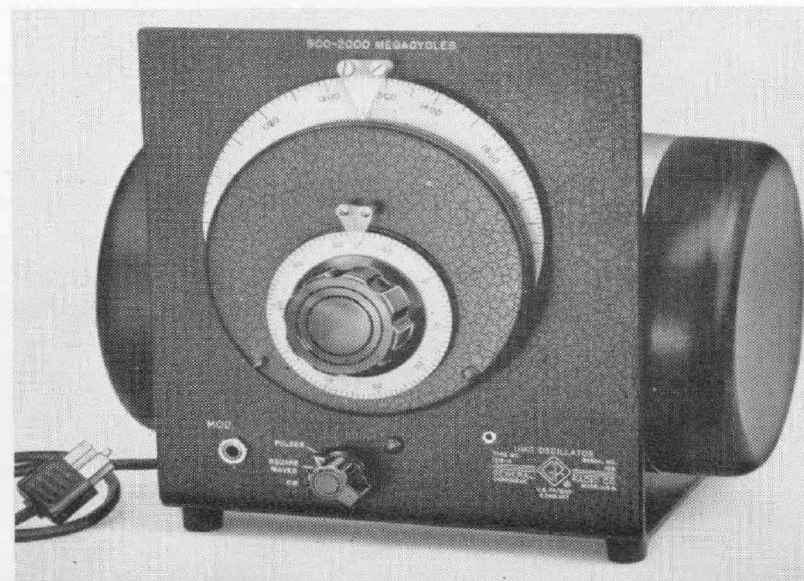
Figure 1. View of the Type 1218-A Unit Oscillator.
