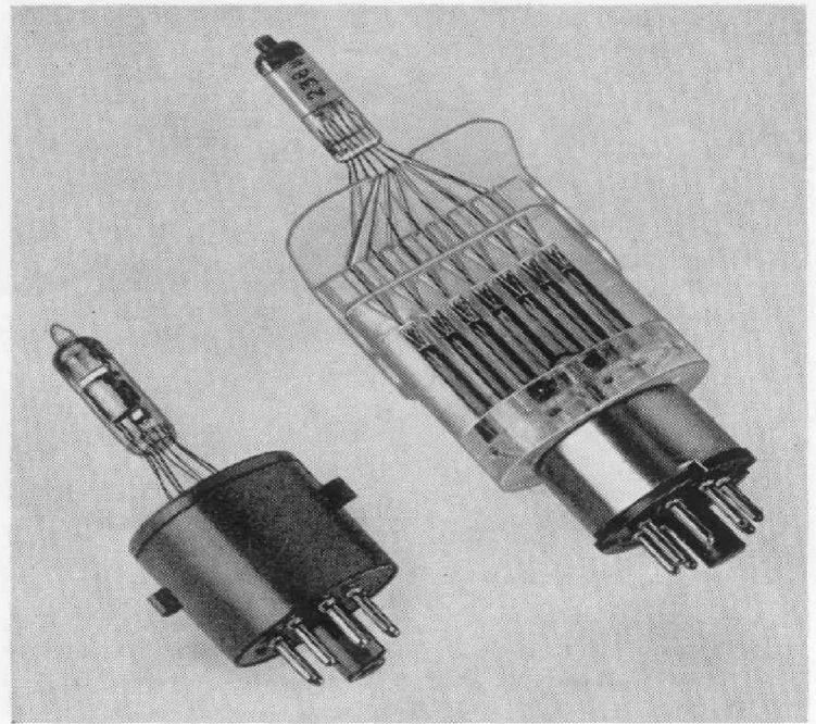
Figure 4. Adaptors for sub-miniature tubes. Flat-press types with up to 7 leads are tested in the Type 561-415-2 Adaptor with a comb-like structure for selecting and guiding the leads into the spring contacts. Eight-wire sub-miniar tubes are tested in the round Type SOA-3 Adaptor, which has provision for locking the leads into the socket. Both types plug into the standard octal adaptor.
