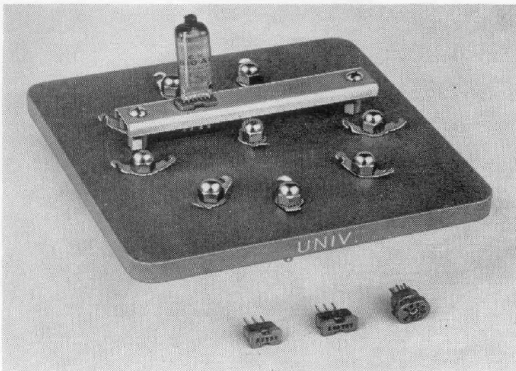
Figure 5 For sub-miniature types with short leads, sockets are supplied which can be mounted on the Universal adaptor. This photograph shows one way of mounting the Type SOT-50 7-pin socket (for flat-press tubes) on a Universal adaptor. In the foreground are shown, left to right, Type SOT-46 for 5-pin tubes, Type SOT-49 for 6-pin tubes, and Type SOT-48 for 8-wire sub-minar tubes.
