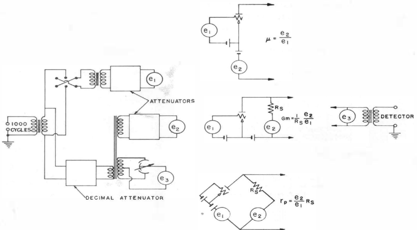
Figure 2. Elementary schematic diagram of the circuits used in the vacuum-tube bridge.
