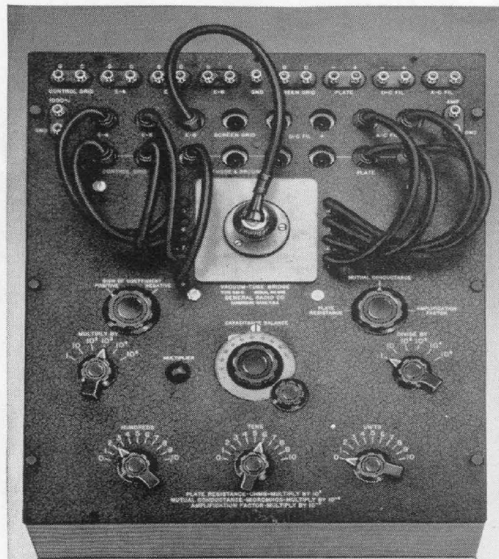
Figure 1. Panel view of the vacuum-tube bridge with adaptor and tube plugged into test position.
