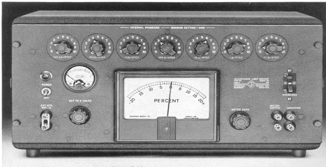
Figure 1. Panel view of the Type 1652-A Resistance Limit Bridge. Per cent deviation is indicated on the large meter, with its open, easily read scale.
