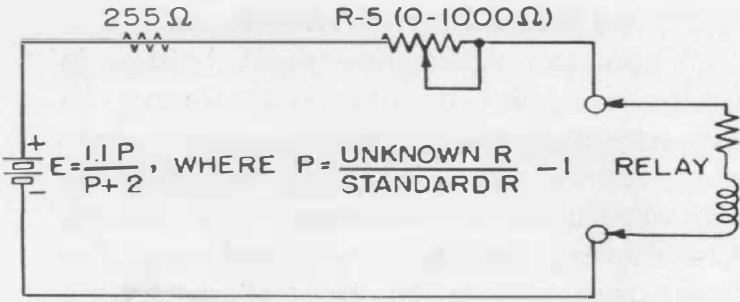
Figure 3. Equivalent circuit of the bridge voltmeter, showing method of connecting on external relay.
