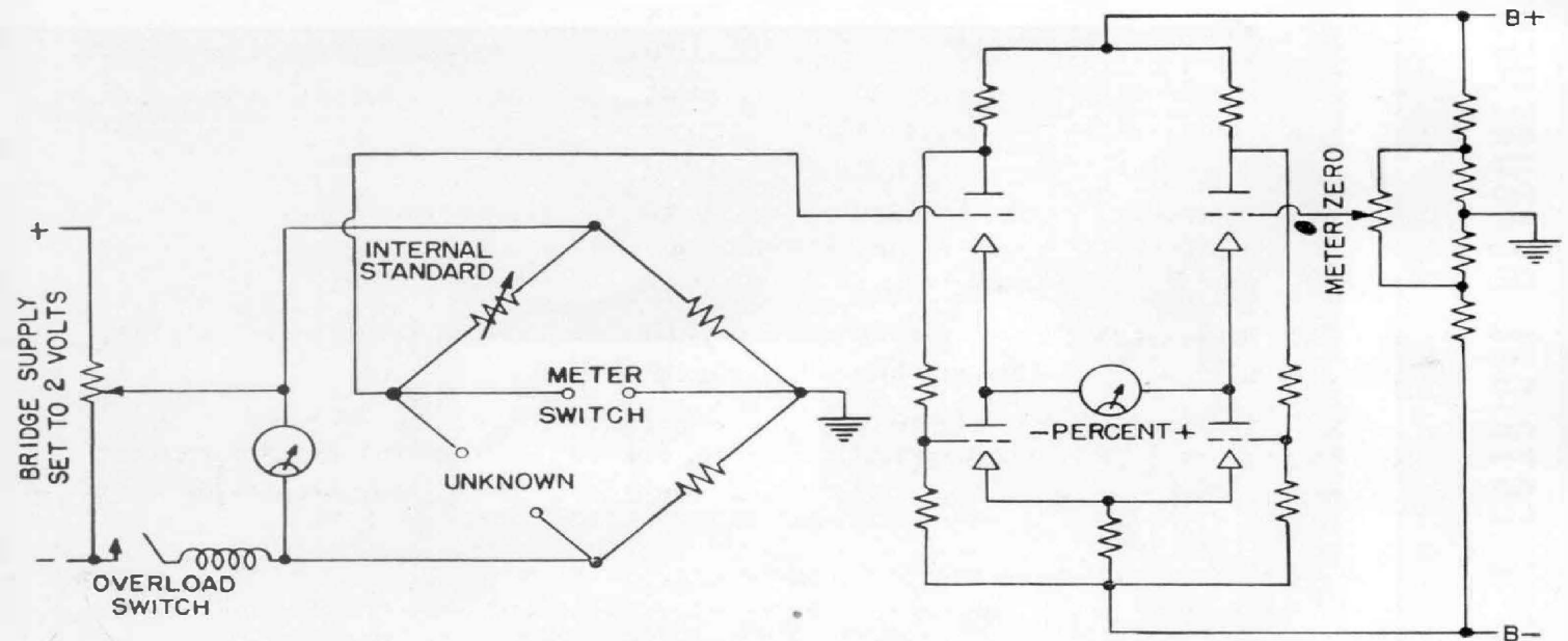
Figure 2. Elementary schematic circuit diagram of the limit bridge.
