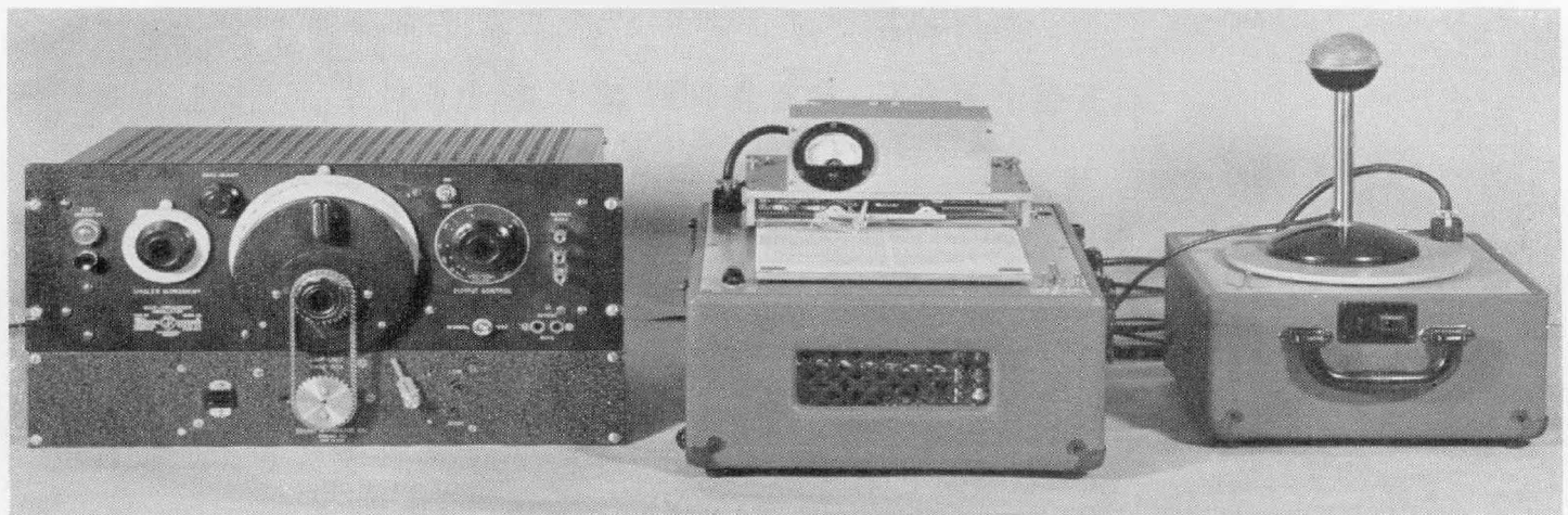
Figure 2. Complete assembly for measuring frequency response characteristics.
