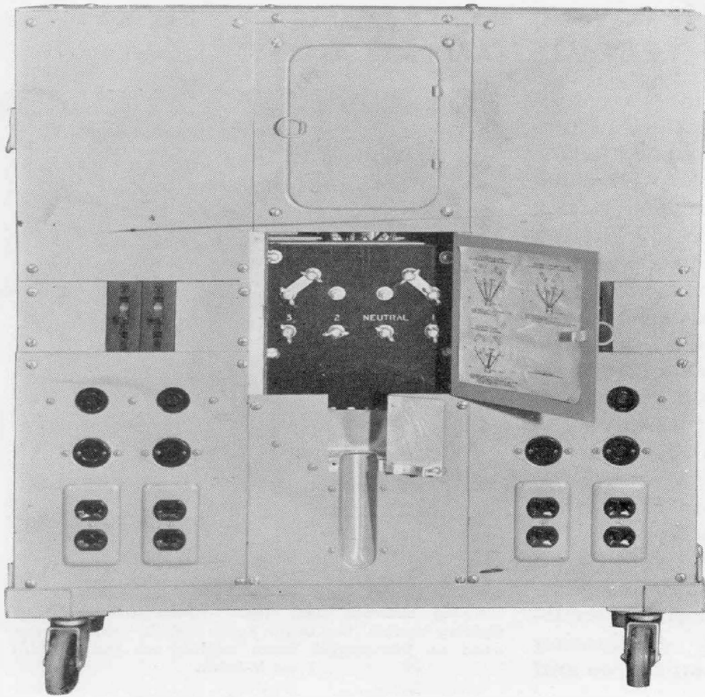
(Left) Figure 2. Rear view of the unit showing camera outlets, duplex outlets, and the panel for input connections, with links for adapting the circuit to different types of power supply.
