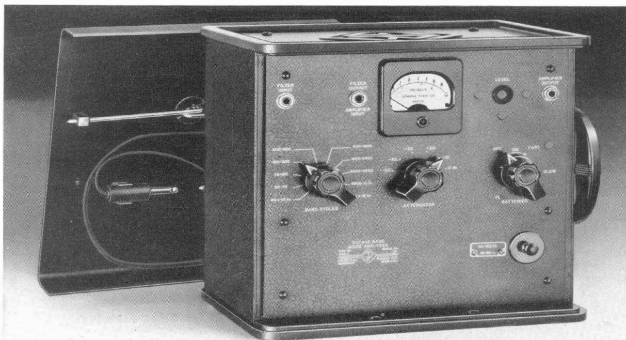
Figure 1. View of the Type 1550-A Octave-Band Noise Analyzer with cover removed to show panel.
