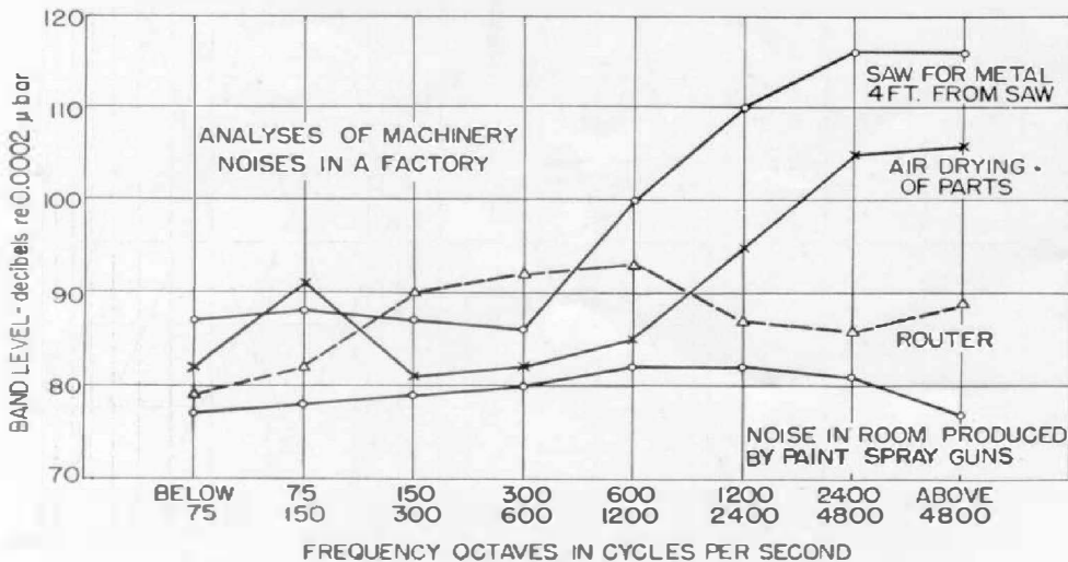
Figure 4. Octave-Band frequency analysis of noise produced by machines in a factory.
