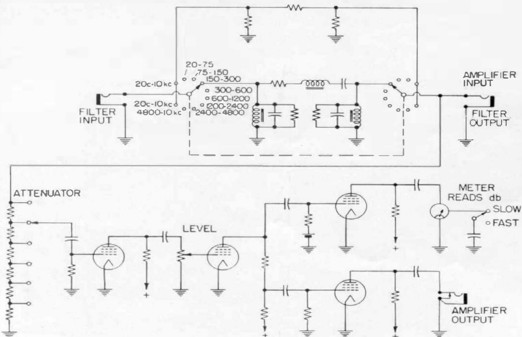
Figure 2. Elementary schematic circuit diagram of the analyzer.
