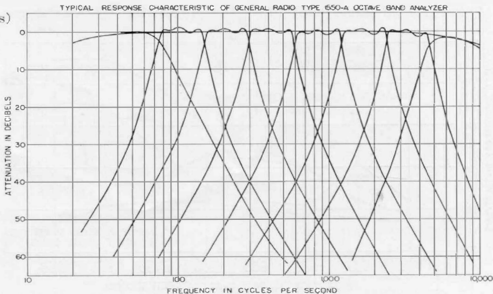
Figure 3. Typical response characteristic of the Type 1550-A Octave-Band Noise Analyzer.
