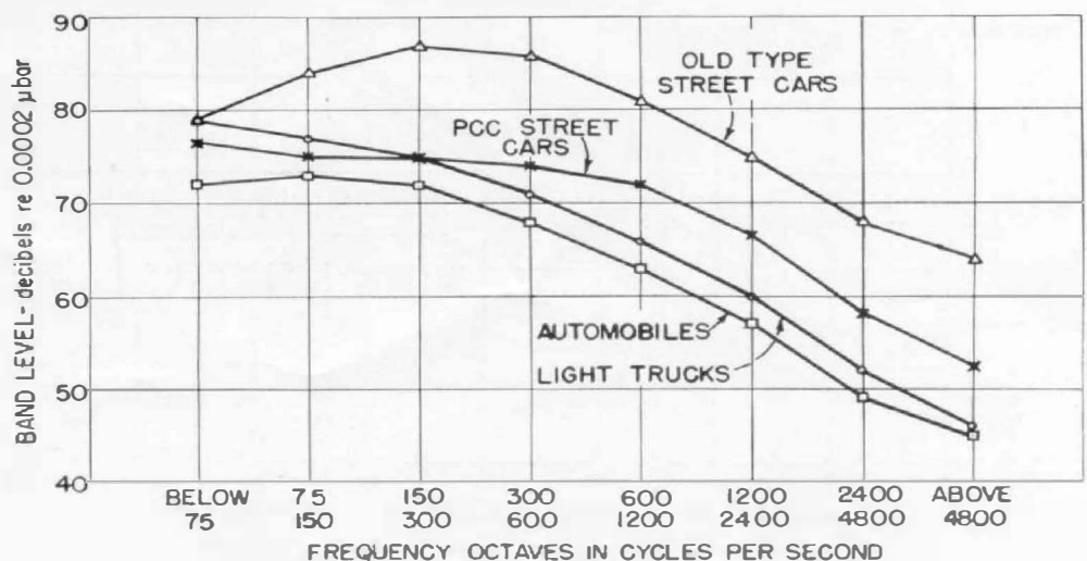
Figure 5. Results of analysis of vehicle noise made with an octave-band analyzer at a distance of 20 feet from the vehicles.
