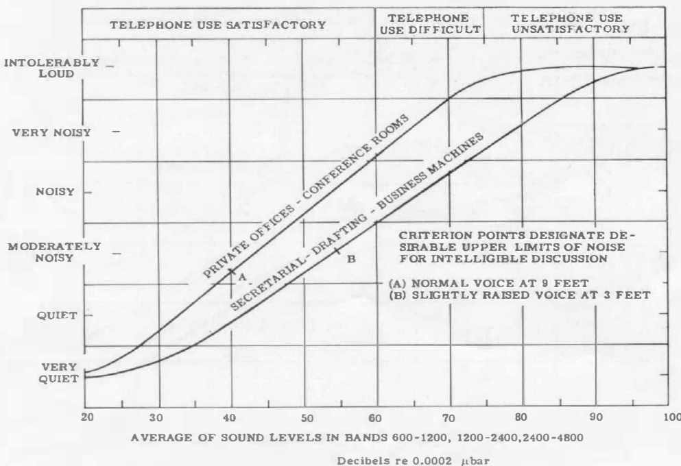
Figure 6. Rating chart for office noises. Data were determined by an octave-band analysis and correlated with subjective tests. (Courtesy Beranek and Newman.)
