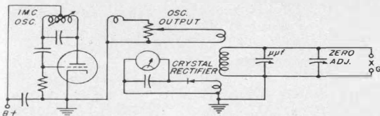
Figure 3. Simplified schematic circuit diagram of the R-F Capacitance Meter.
