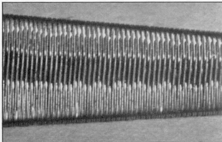
Figure 3. Close-up view of an Ayrton-Perry non-inductive winding on a tapered form.
