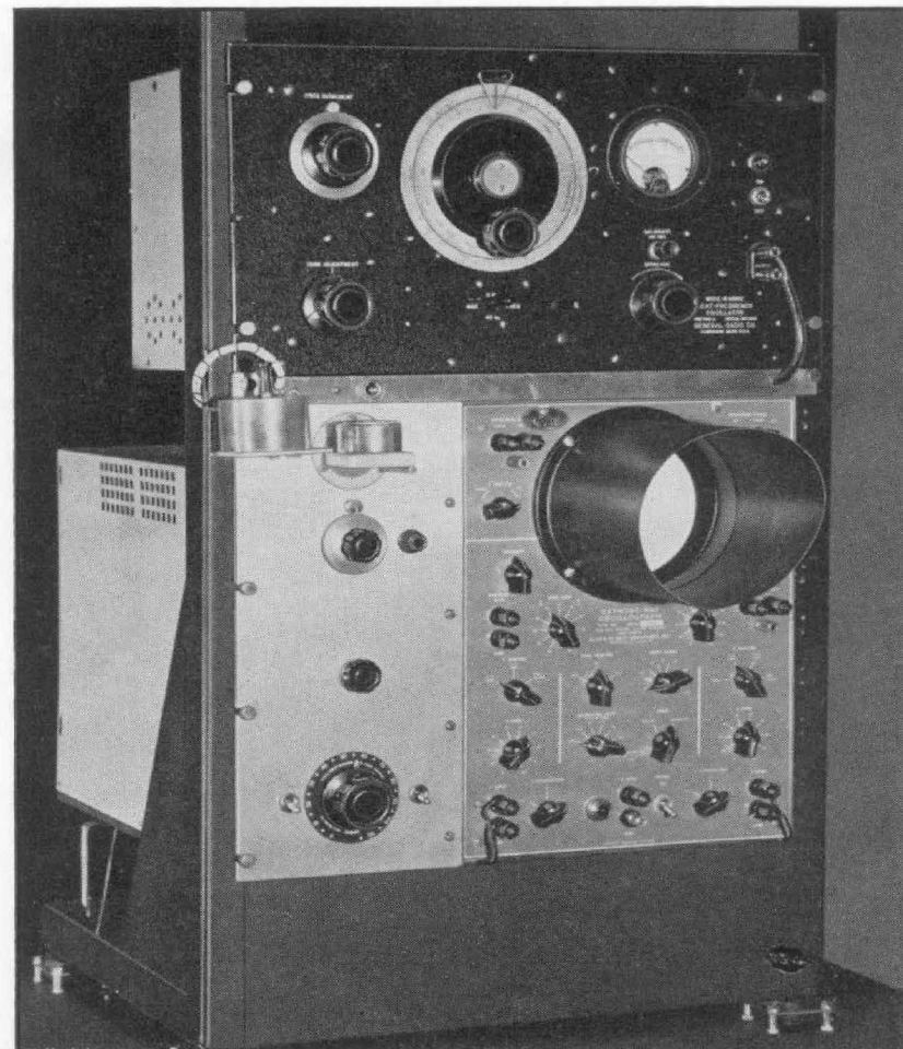
Figure 1. Panel view of the crystal mode indicator.
