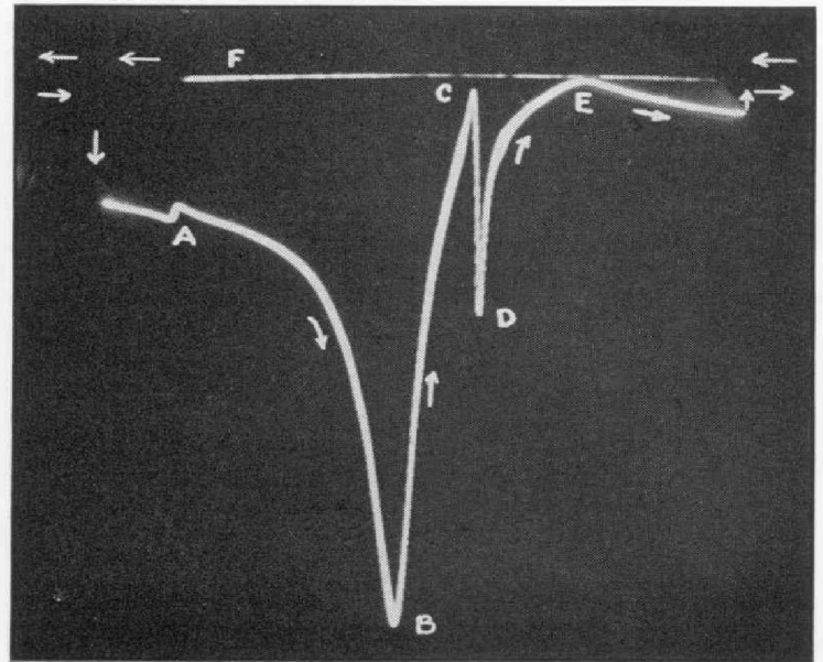
Figure 4. Oscillogram of the response of a quartz plate with two spurious response frequencies.
