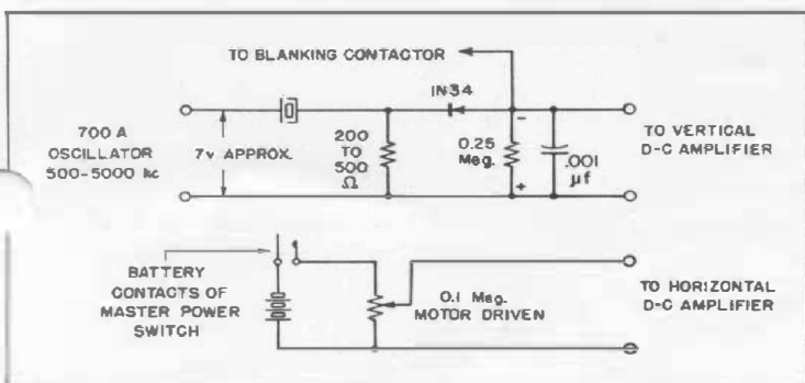
Figure 3. Schematic diagram of the electrical circuit.
