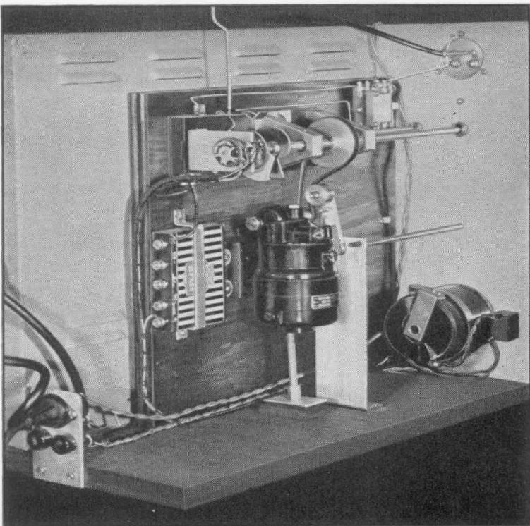
Figure 2. Rear view, showing the motor drive and frequency-sweeping capacitor.
