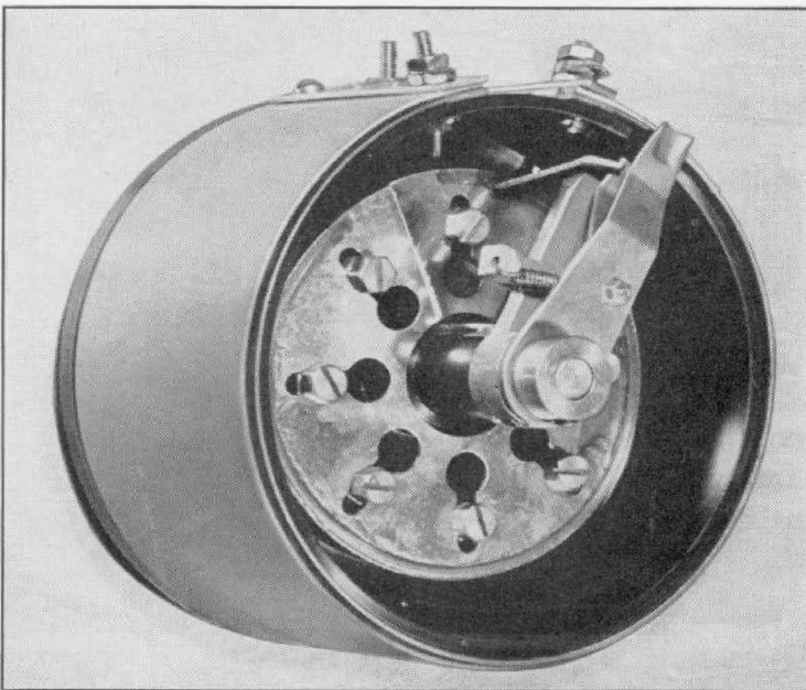
Figure 2. A 5-inch-barrel potentiometer with justifying mechanism. This resistor is used in the Type 650-A Impedance Bridge.
