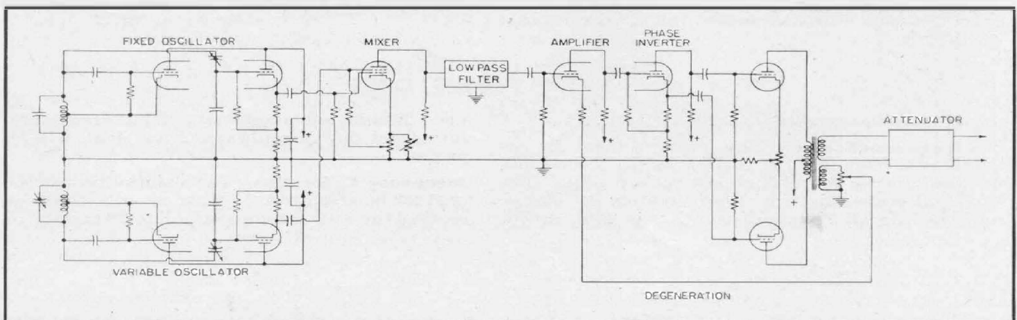
Figure 2. Elementary schematic circuit diagram of the Type 1304-A Beat-Frequency Oscillator.
