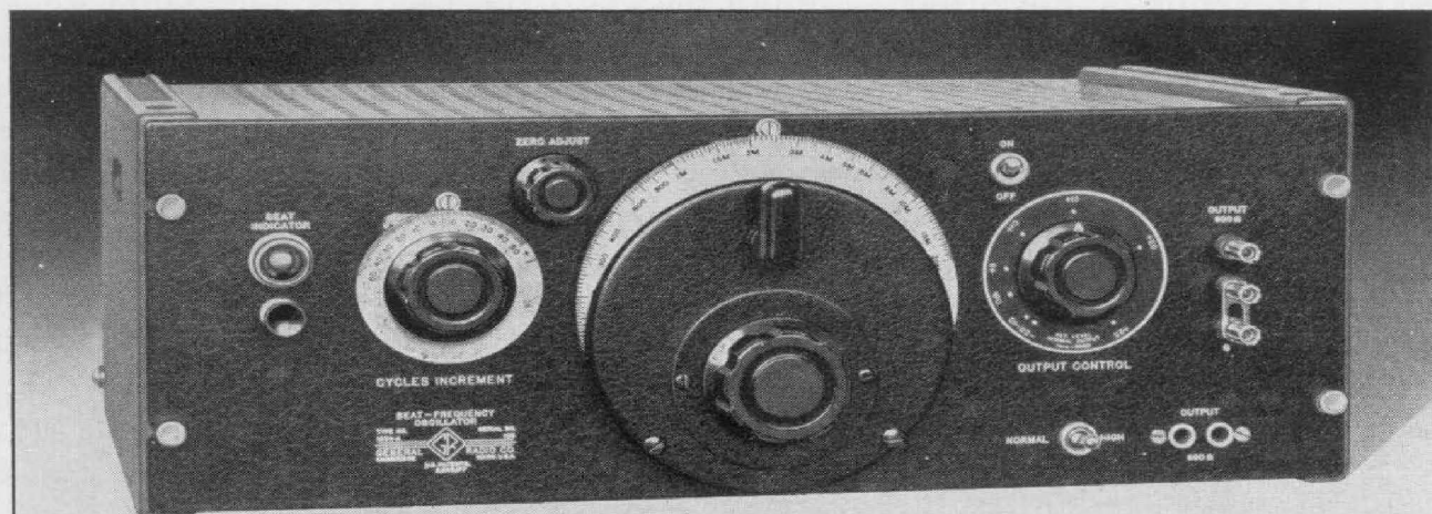
Figure 1. Panel view of the Type 1304-A Beat-Frequency Oscillator. New features include an illuminated, precision-type, main dial, and an incremental frequency dial with a range of -50 to +50 cycles.
