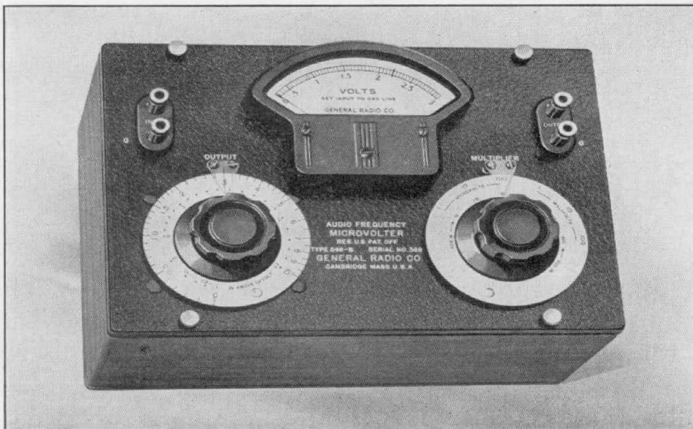
Figure 1. Panel view of the Microvolter. Photograph shows previous model, Type 546-B. New model differs very little in appearance.
