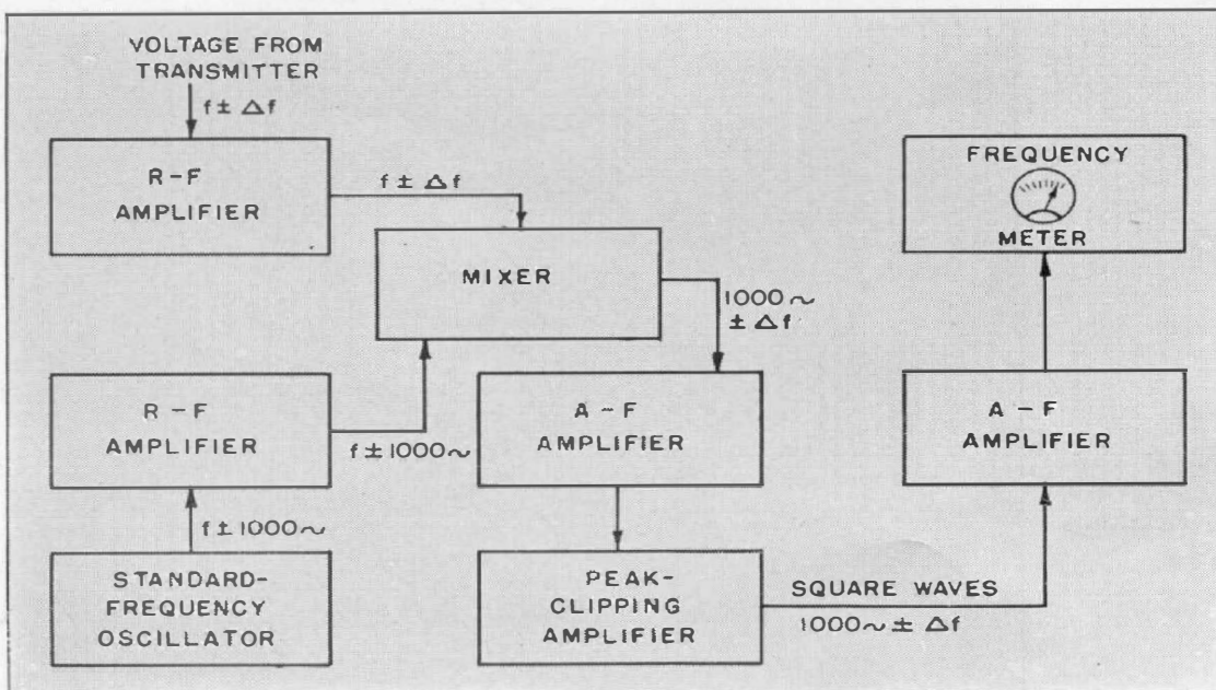
Figure 2. Functional block diagram showing the operation of the frequency-deviation monitor.
