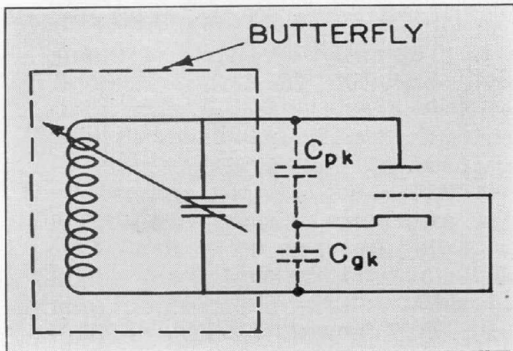
Figure 3. Basic r-f oscillator circuit.
