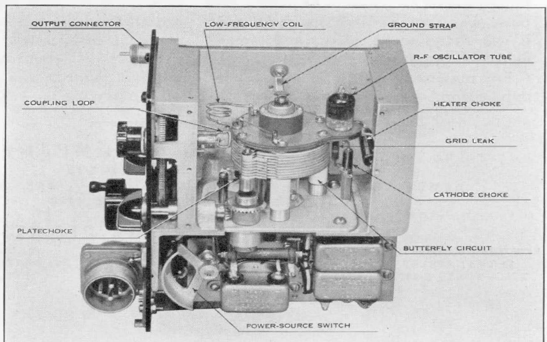
Figure 4. Interior view of the instrument with shields removed.
