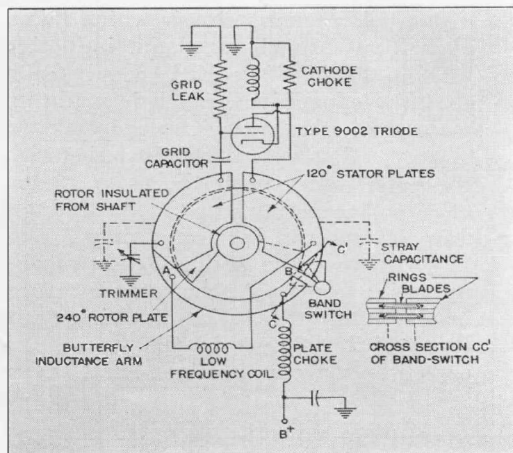
Figure 2. Diagram of the r-f oscillator showing general construction of the butterfly and the band switch.
