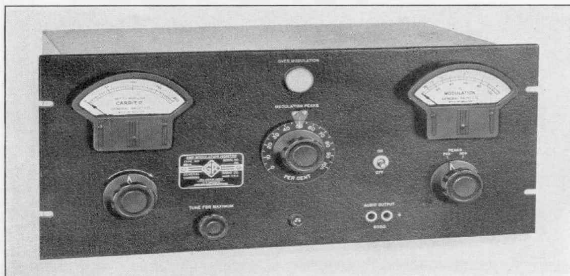
Figure 3. Panel view of the Type 1931-A Modulation Monitor.
