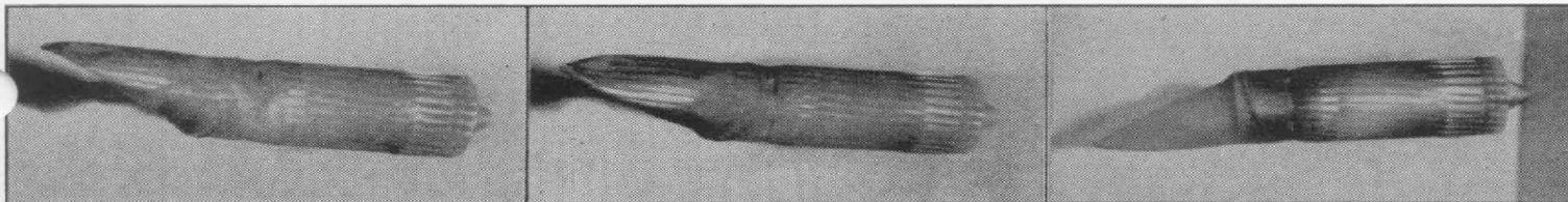
FIGURE 4. Photographs of three rounds of ammunition showing both yaw and erratic behavior of windshields.
