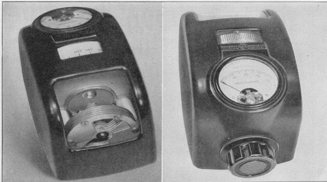
FIGURE 1. Two views of the TYPE 1140-A U-H-F Wavemeter. At the front, the butterfly is seen through a transparent window; at the rear, both the resonance indicator and the frequency scale can be read as the tuning control is turned.
