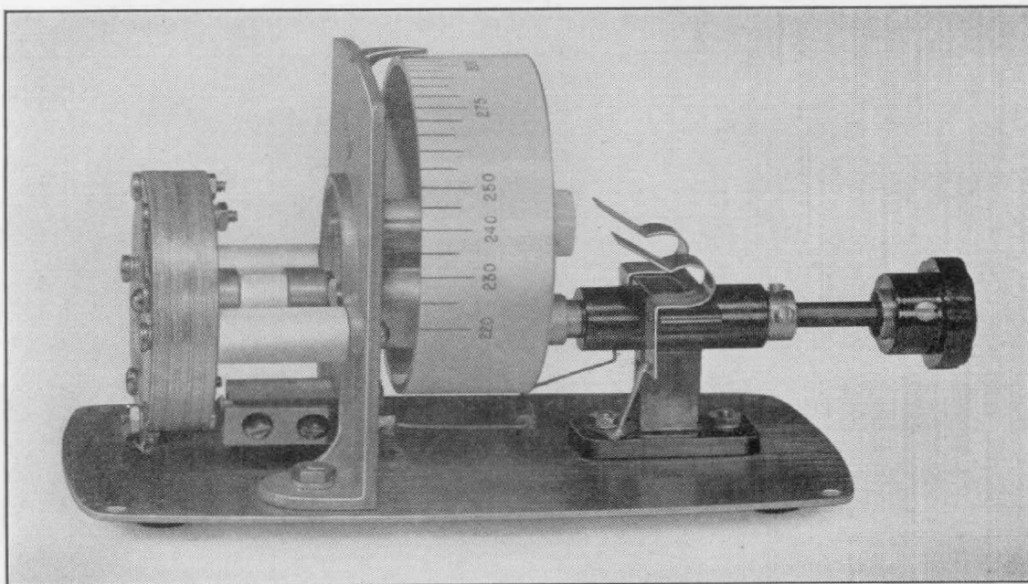
FIGURE 2. View of the interior of the wavemeter with case removed. The cartridge-type crystal detector is mounted in the metal block near the base at the rear of the butterfly. The two clips above the shaft bearing make contact with the terminals of the micro-ammeter, so that both original assembly and removal for servicing are easily accomplished.
