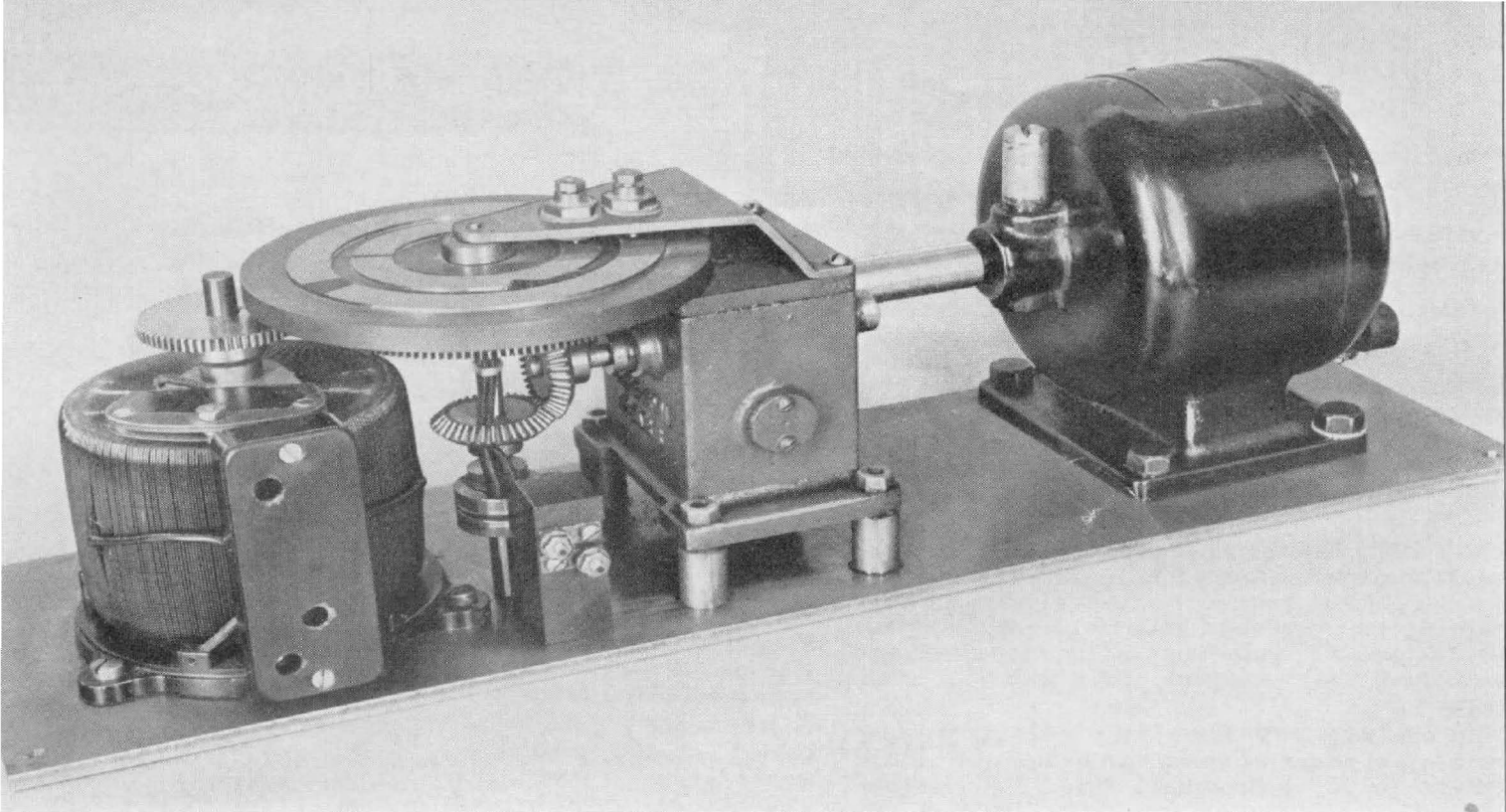
View of a motor-driven Variac with automatic limit attachment.
