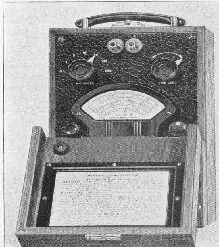
FIGURE 1. View of the voltmeter with cover open.
