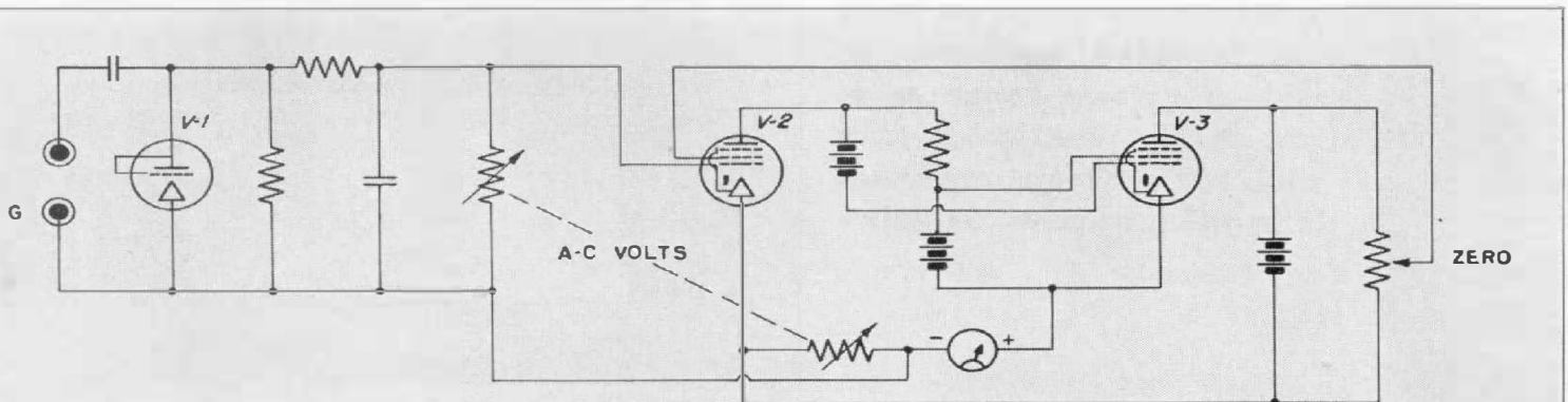
FIGURE 3. Schematic circuit diagram of the TYPE 727-A Vacuum-Tube Voltmeter.
