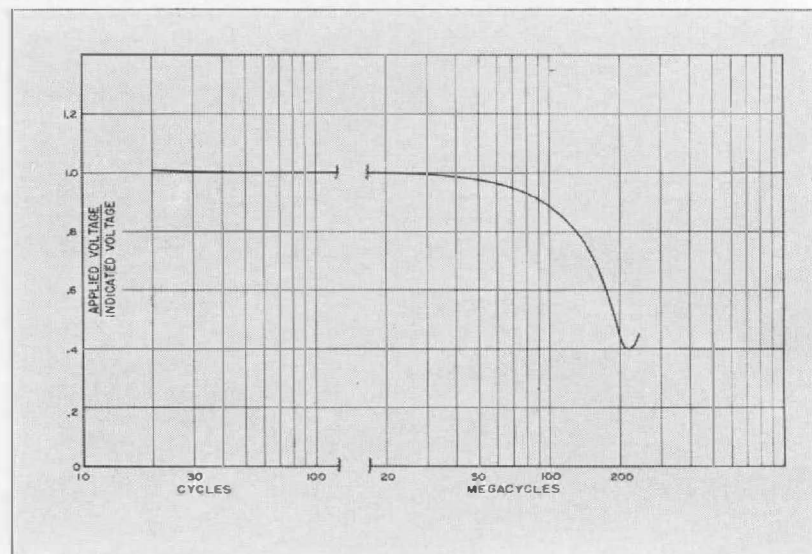
FIGURE 4b (below). Frequency characteristics of the new TYPE 727-A Vacuum-Tube Voltmeter.
