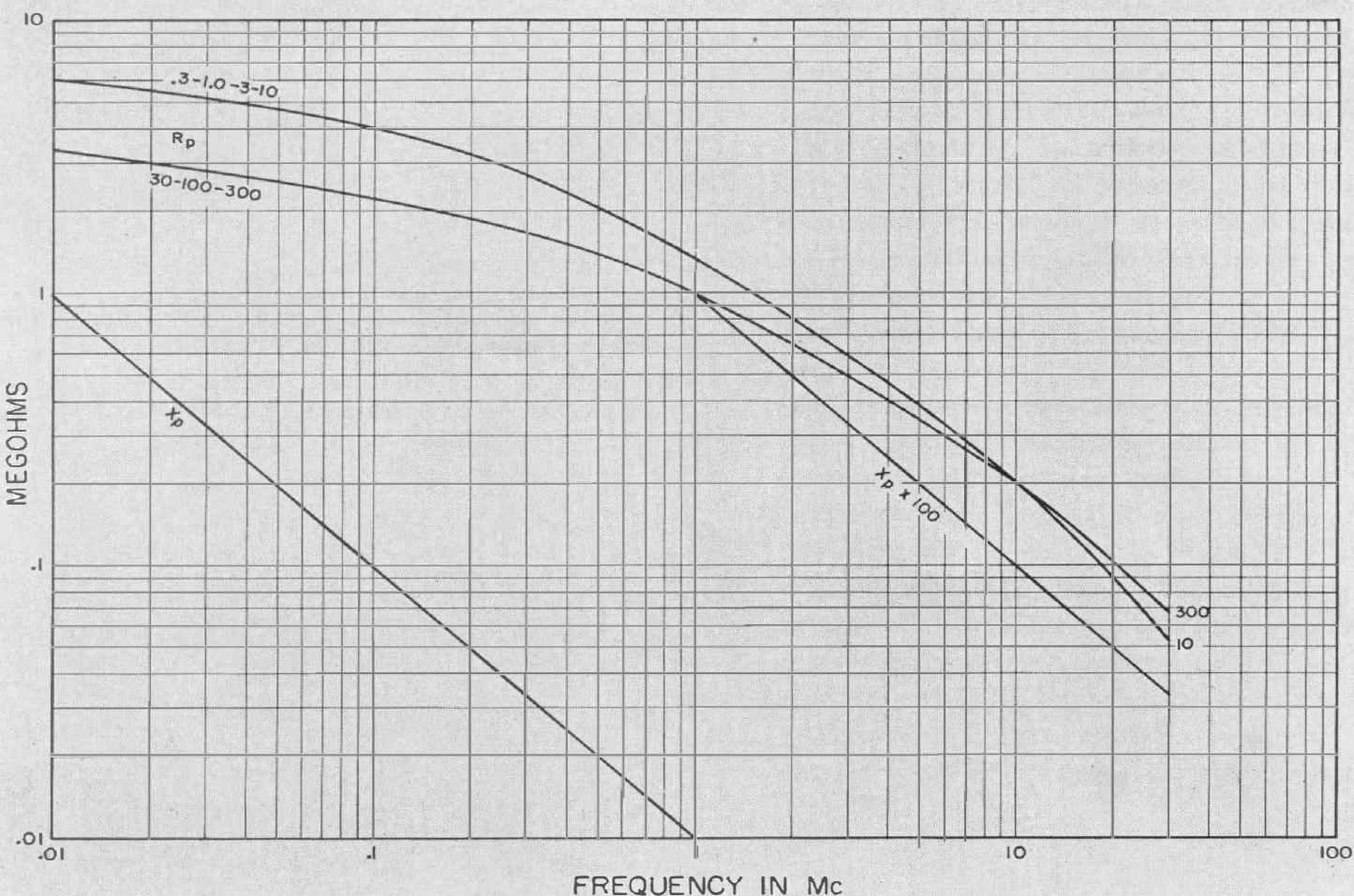
FIGURE 5. Input impedance of the TYPE 727-A Vacuum-Tube Voltmeter as a function of frequency.
