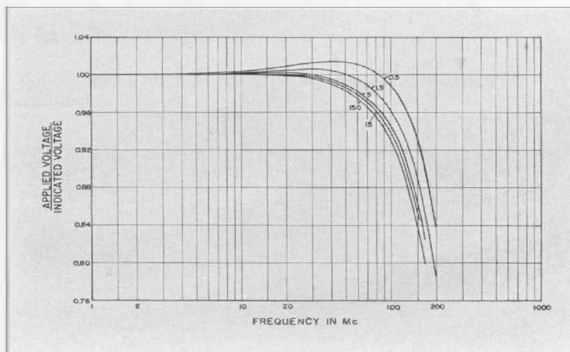
FIGURE 4a (above). Frequency characteristics of the older TYPE 726-A Vacuum-Tube Voltmeter.
