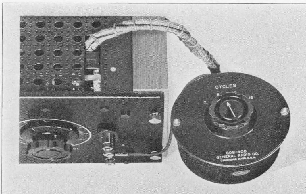
FIGURE 1. Showing a range-extension unit connected to the TYPE 608-A Oscillator. A jack plate is provided in the oscillator, and the only necessary modification is the hole in the cover to admit the plug.
