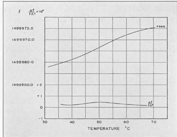
FIGURE 7. Plot of frequency vs. temperature and of temperature coefficient vs. temperature for a production crystal (TYPE 376-L).
