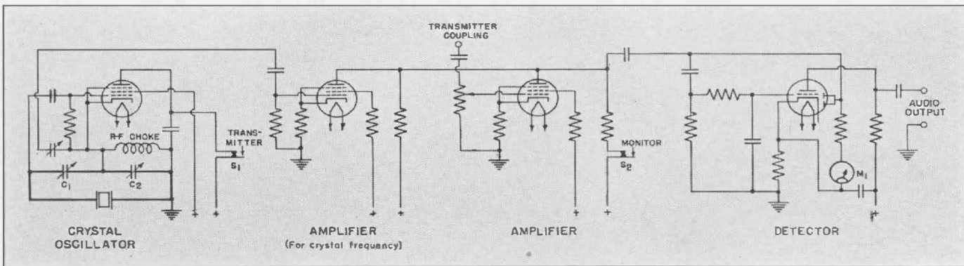
FIGURE 3. Schematic circuit diagram of the TYPE 475-C Frequency Monitor. The meter M_1 in the diode circuit indicates the levels of the signals from the crystal oscillator and the transmitter. Additional contacts (not shown in the diagram) on the push buttons short circuit the meter when neither button is depressed.
