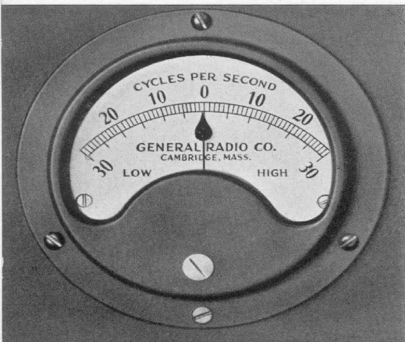
FIGURE 6. Frequency deviations are indicated on this meter, which can be read to better than one-half cycle.
