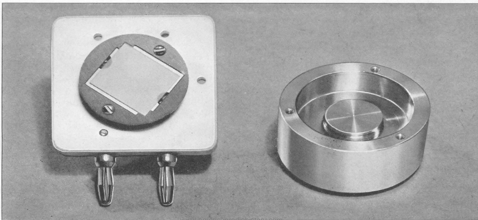
FIGURE 8. This photograph shows the method of mounting the quartz plate so that it is held securely in position without restraining its vibration.
