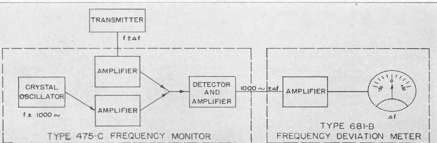
FIGURE 2. Functional block diagram of the monitoring system. The frequency of the monitoring crystal can be either above or below that of the transmitter, since reversing the leads of the indicating meter reverses the direction of the deviation indication.
