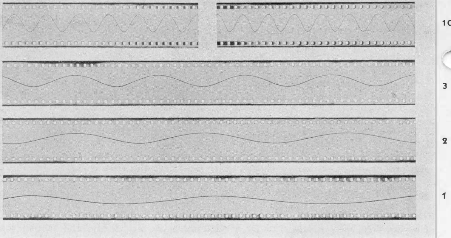
FIGURE 2. Oscillograms of the output voltage of TYPE 608-A Oscillator at low frequencies. Reading from top to bottom the frequencies are 10, 3, 2, and 1 cycle per second. These waveforms were photographed with a TYPE 651-A Camera.
