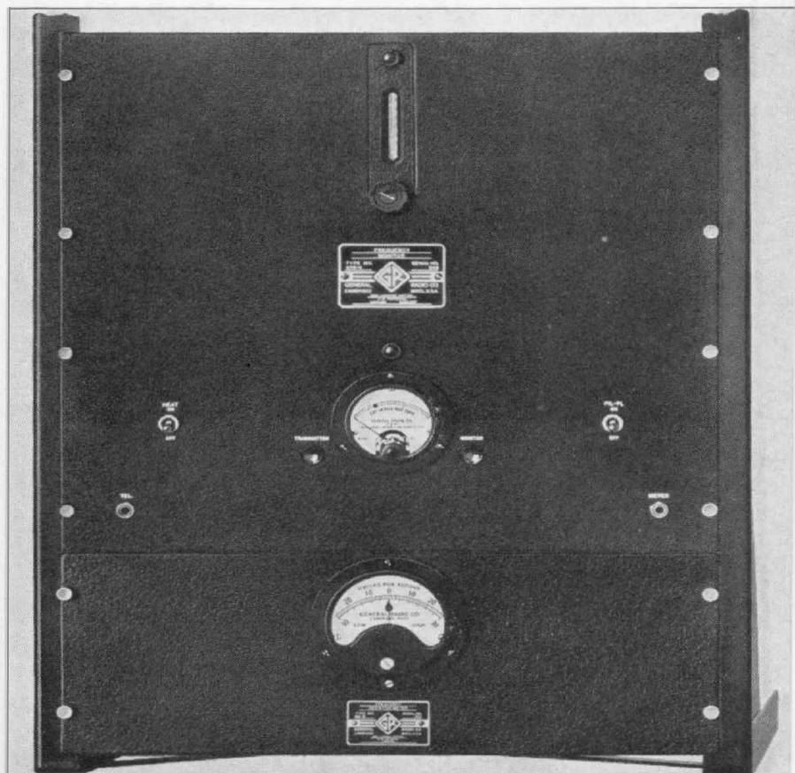
FIGURE 1. Panel view of the broadcast frequency monitor.
