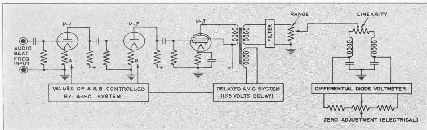
FIGURE 5. Schematic circuit diagram of the TYPE 681-B Frequency Deviation Meter. The automatic volume control eliminates the need for a manual input control.
