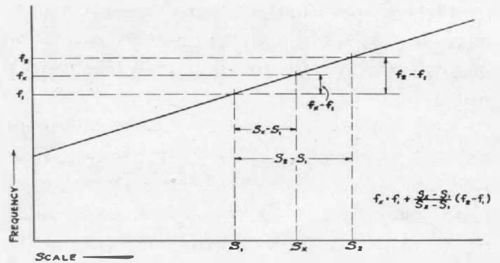
Illustrating method of interpolation between standard-frequency harmonics
