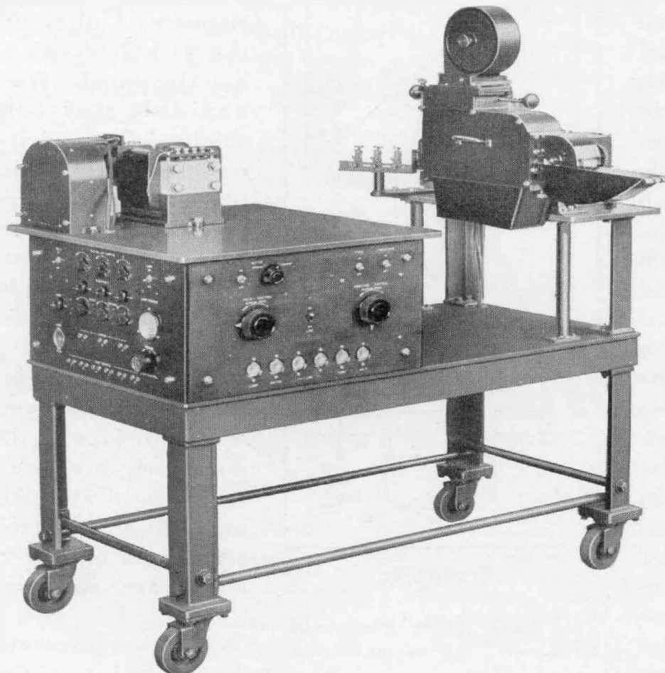
A three-element camera oscillograph with the self-developing feature
