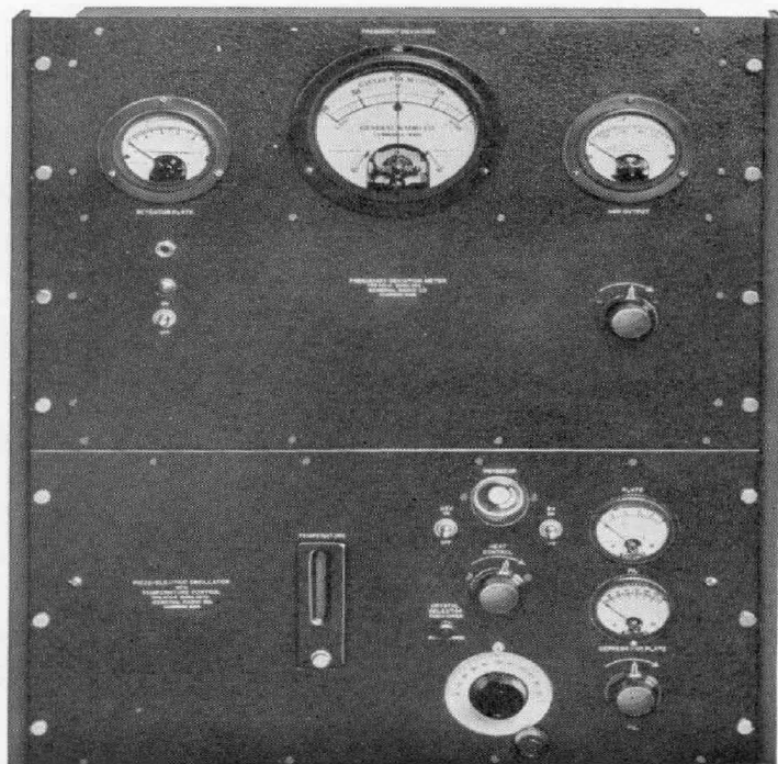
FIGURE 1. The frequency monitor consisting of a TYPE 575-D Piezo-Electric Oscillator and a TYPE 581-A Frequency Deviation Meter
