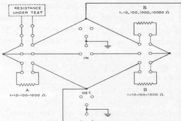
FIGURE 2. Schematic diagram for the measurement of resistance by the Wheatstone Bridge
