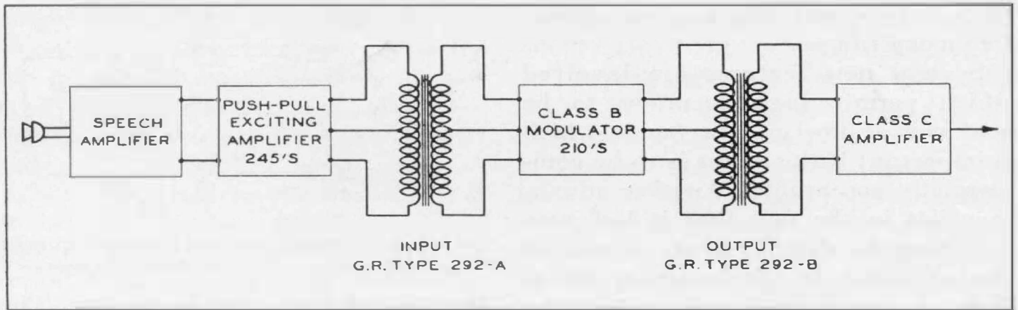
Schematic diagram for a low-power amateur phone transmitter utilizing General Radio TYPE 292 Transformers in a "Class B" Modulator
