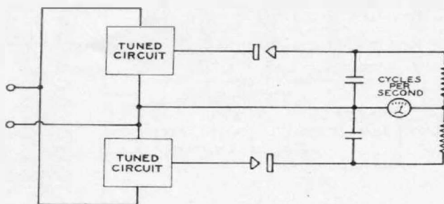
FIGURE 3. Schematic diagram for the frequency indicating element of the deviation meter
