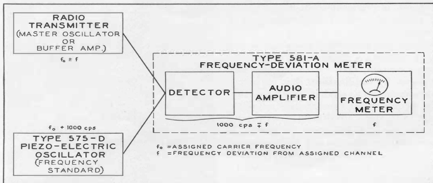
FIGURE 2. Schematic diagram for the frequency monitor. The "frequency standard" is operating at a frequency 1000 cps above that of the carrier. When operating 1000 cps below the carrier the beat frequency involved in the deviation meter is (1000 \pm f)
