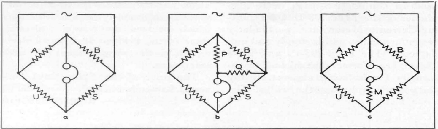
FIGURE 3. Practically all bridge networks are elaborations of these three basic circuits. The letters a, b and c refer to the second column of Table I
