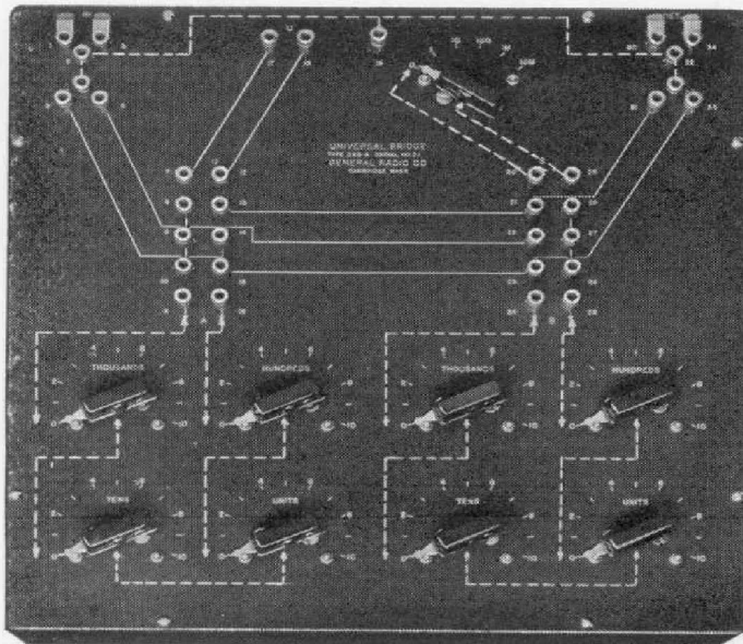
FIGURE 1. Panel view of a TYPE 293-A Universal Bridge. Dotted lines were drawn in after the photograph was taken
