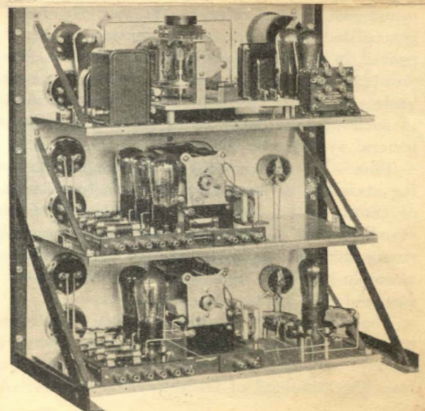
THE TWO-STAGE MULTI-VIBRATOR AND TIMING AMPLIFIER FOR THE NEW FREQUENCY DETERMINATION EQUIPMENT
