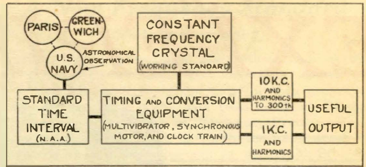
FIGURE 4. AN OUTLINE CHART FOR THE GENERAL RADIO COMPANY'S FREQUENCY-DETERMINATION SYSTEM
