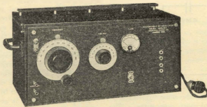
FIGURE 6. THE TYPE 584 A.C. PORTABLE R. F. OSCILLATOR. COILS ARE PLUGGED INTO THE FOUR JACKS AT THE RIGHT
