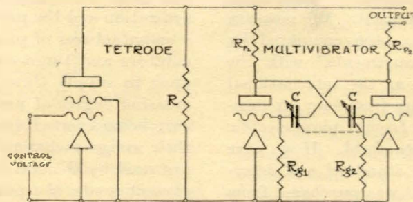
FIGURE 5. SCHEMATIC CIRCUIT OF THE MULTIVIBRATOR AND ITS AMPLIFIER
