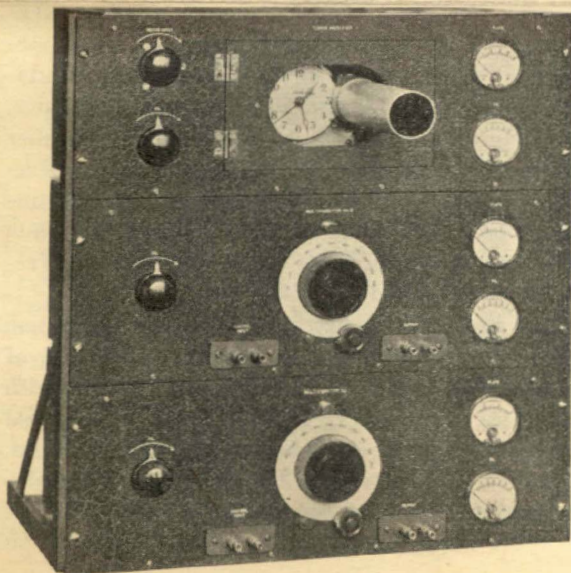
THE TWO-STAGE MULTI-VIBRATOR AND TIMING AMPLIFIER FOR THE NEW FREQUENCY DETERMINATION EQUIPMENT
