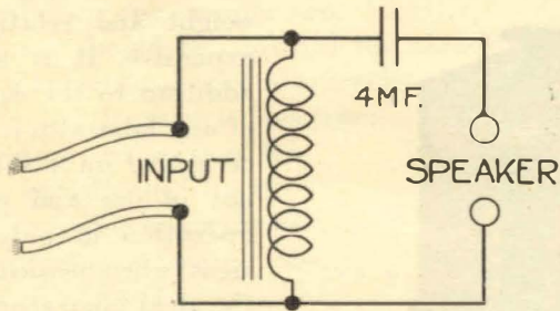
FIGURE 8. WIRING DIAGRAM FOR THE TYPE 587-C SPEAKER FILTER
