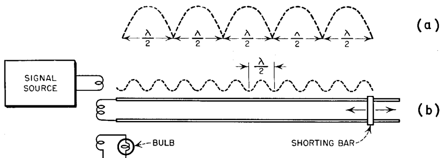
TYPICAL LECHER WAVEMETER FIG. 1
