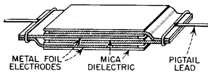
TYPICAL MICA CAPACITOR CONSTRUCTION FIG. 2
