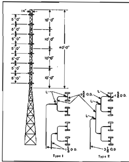
Figure 9 Eight loop tower and feed line arrangements. In this setup a separate line is used to feed each group of four loops, two lines being joined in proper phase at the ground level or in a transmitter house. L = \frac{1}{4} wave matching transformer.
