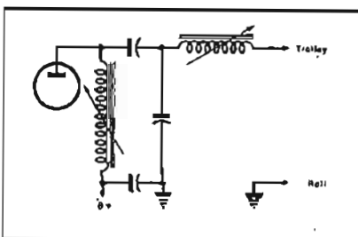
Figure 3 The impedance-matching network designed to couple the power-amplifier tubes to the power line, a system used because of the high transformation ratio of 7,000 to 2.5 ohms.
