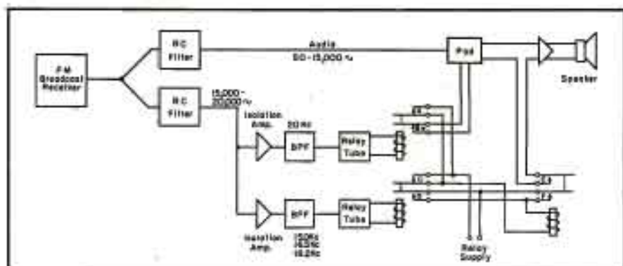
Figure 3 Block diagram of the FM supersonic control system; *pad may be adjusted so that control \beta will boost gain 5 to 15 db or open circuit as required.
