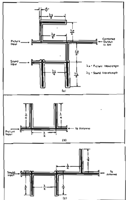
Figures 11 a, b and c In (a) appears a schematic of a basic TV diplexer system. The equivalent picture circuit of the diplexer is illustrated in (b) and in (c) appears the equivalent sound circuit.
