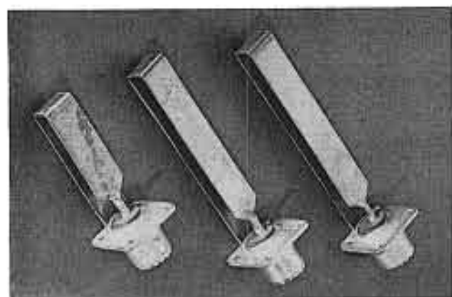
Figure 5 Three loops used with 160-mc cavity filter.
