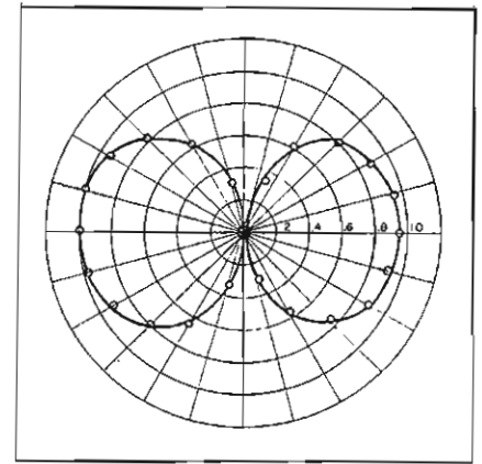
Figure 8 Vertical radiation pattern of the triangular loop.
