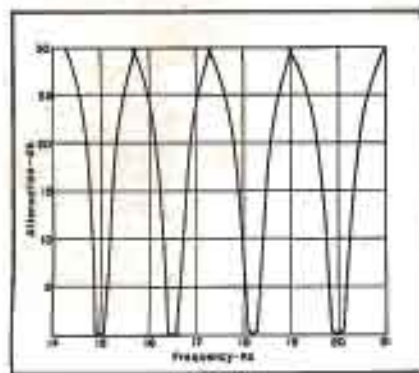
Figure 2 Selectivity characteristics of supersonic-control filters used in the receiver.
