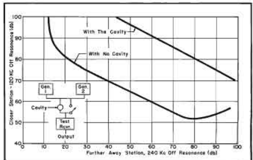
Figure 8 Plot of intermodulation interference measurements with and without cavity filter. (Reference level: .5 microvolt at receiver input, for 20 db quieting, assumed 0 db.)
