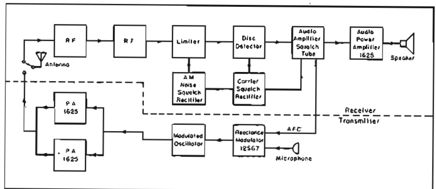
Figure 4 Block diagram of the 100-kc FM transmitter-receiver.
