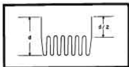
Figure 2 Peak cw voltage adjusted to 1/2 peak-pulse voltage.
