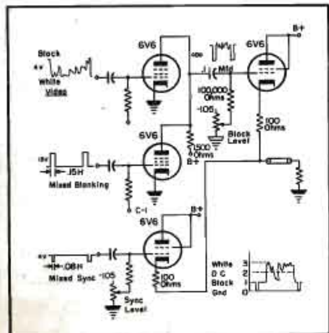
Figure 3 Line mixing amplifier: output circuit.
