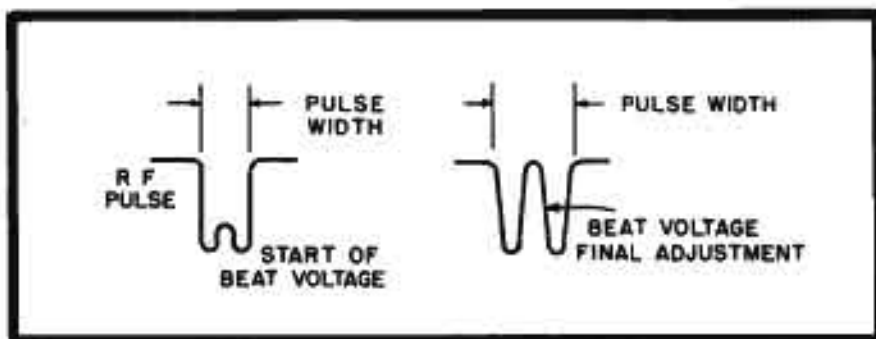
Figure 1 Cw voltage beating with pulse voltage.
