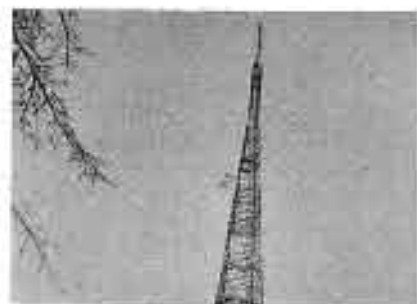
TV tower of WDTV, Pittsburgh, Pa. Structure, 500' high, weighs 100 tons, and is 60' square at the base, tapering to a 5 1/2' square. (Courtesy Blaw-Knox)
