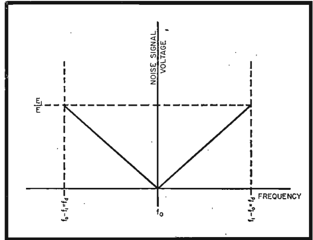
Figure 2 Noise voltage generated by an adjacent signal of frequency f_1 , magnitude E_1 , on a carrier of frequency f_0 and magnitude E . Receiver frequency deviation, f_d .
