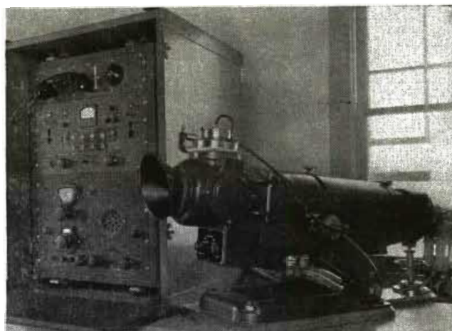
Control equipment of a semi-portable FTR h-f direction finder. Uses a horizontal U-line transmission line system. Overall d-f frequency range is 2 to 10 mc. Receiver has a 1.5 to 30 mc 4-band range.
