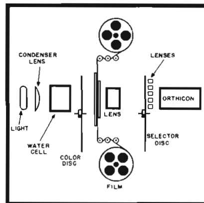
Figure 14a Projection viewing color television receiver also built by CBS for their color television sets. Image of about 22" width is provided.
