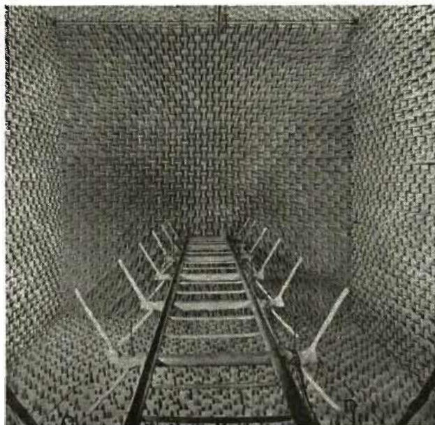
Above, a view of the echo-free chamber that was built to simulate atmospheric conditions existing at 1,000' to 3,000' above earth. The walls are almost perfectly absorbing; less than 1/1,000 of the sound that strikes a wall is reflected. The room was developed under the supervision of Dr. Leo L. Beranek, as head of the electroacoustic laboratory. H. P. Sleeper, Jr., was co-inventor of the room. The room has been used to study loudspeakers, microphones, and headphones. It is equally good at frequencies between 70 and 20,000 cps. Density of the fibrous glass material and the dimensions must be critically determined once the lowest frequency at which 99% or better absorption is decided upon.
