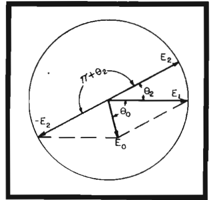
Figure 5 Vector diagram showing subtraction of two voltage vectors E_1 and E_2 displaced \theta_2 radians, and resulting vector E_0 displaced \theta_0 radians from E_1 .
