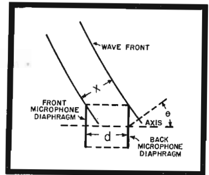
Figure 4 Relation between X , the distance between two instantaneous values of an assumed sound wave from the horn, which are acting on the front and back microphone diaphragms simultaneously; d , the separation distance between diaphragms on the microphone axis; and \theta , the angle between the axis and the direction of wave motion.
