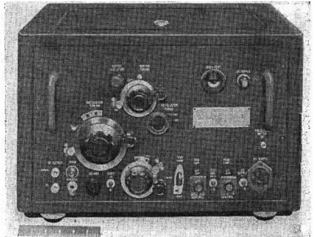
Figure 4 Frequency shift exciter of radioteletype system.
