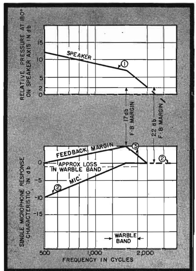
Figure 8 Response of single microphone (2) required to maintain a minimum of 17-db feedback margin (3) in the warble band, using a horn loud-speaker with average response as in (1), and resulting loss.
