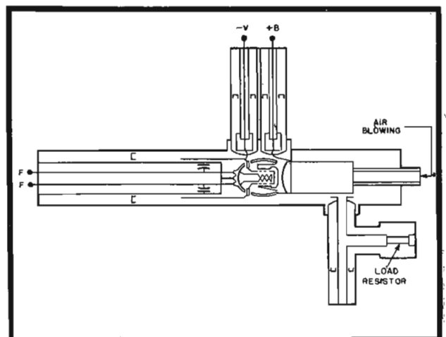
Figure 13 Circuit of test oscillator using an air-cooled version of the 6C22, the L600NR. Plate and grid-bias voltage are brought in through quarter-wave chokes. Cathode circuit is piston tuned, while the plate is adjusted for half-wavelength open-line operation.
