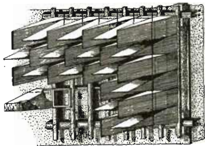
Wedge-shaped fibrous-glass structures that lined the wall of a sound room built in the Cruft Building of Harvard University during the war for NDRC research. There were 20,000 of these wedges in the room, known as the anechoic chamber (without echo).
