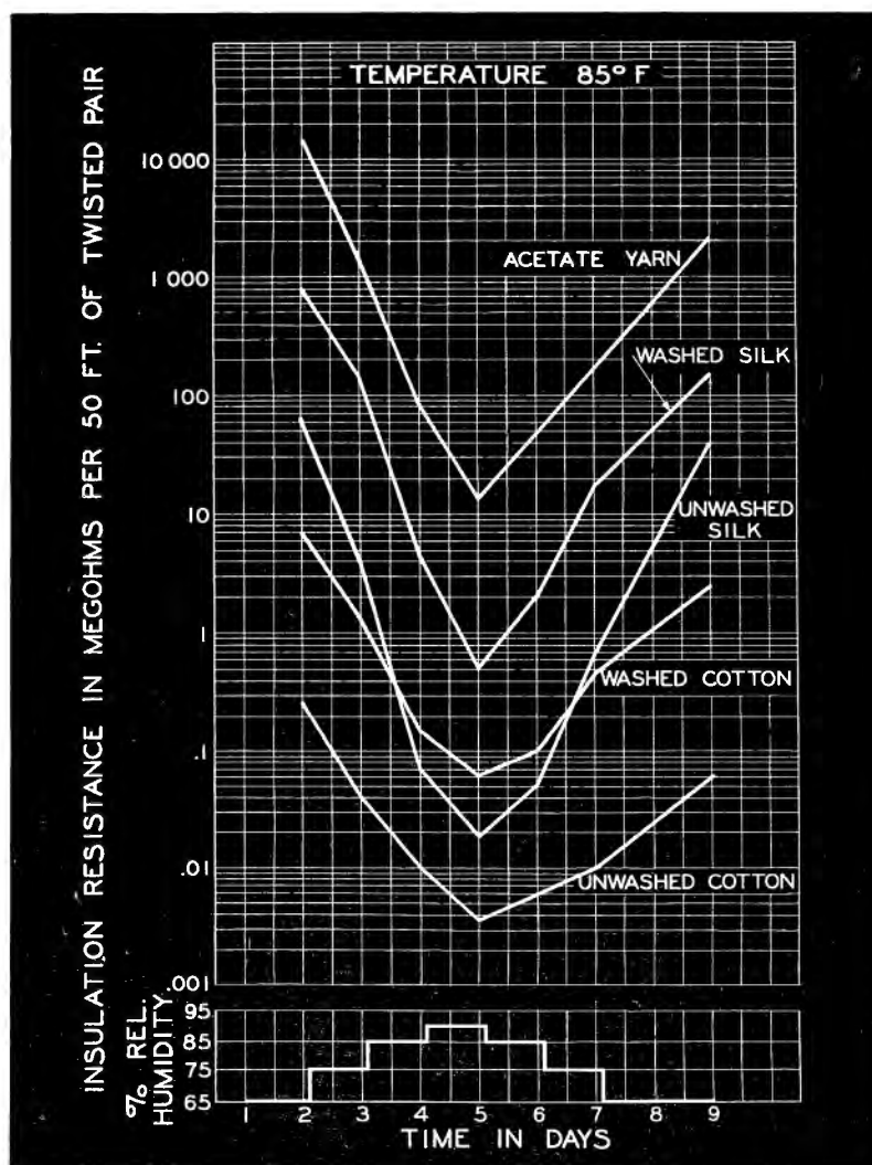
Figure 3 The characteristics of various types of substitute wire coverings.
