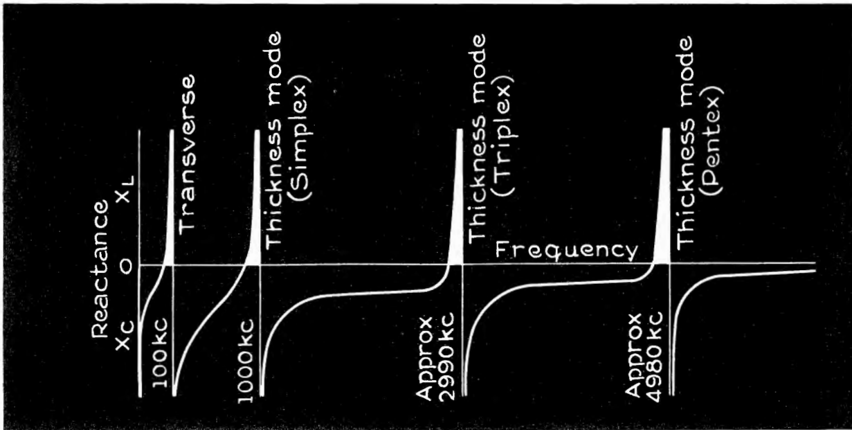
Figure 9 The frequency-reactance characteristics of quartz crystal, showing the various modes of oscillation.
