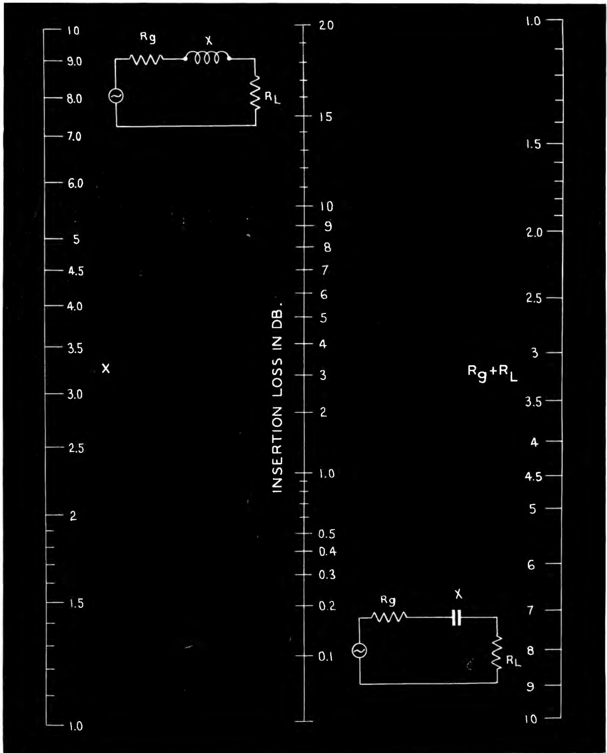
Figure 2 The insertion loss due to series reactance can be computed from this chart.
