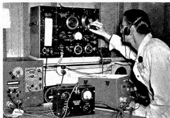
General Radio standard-signal generator and output meter in use in the radio test and repair shop at Pan American Airways' hangar at LaGuardia Field.
