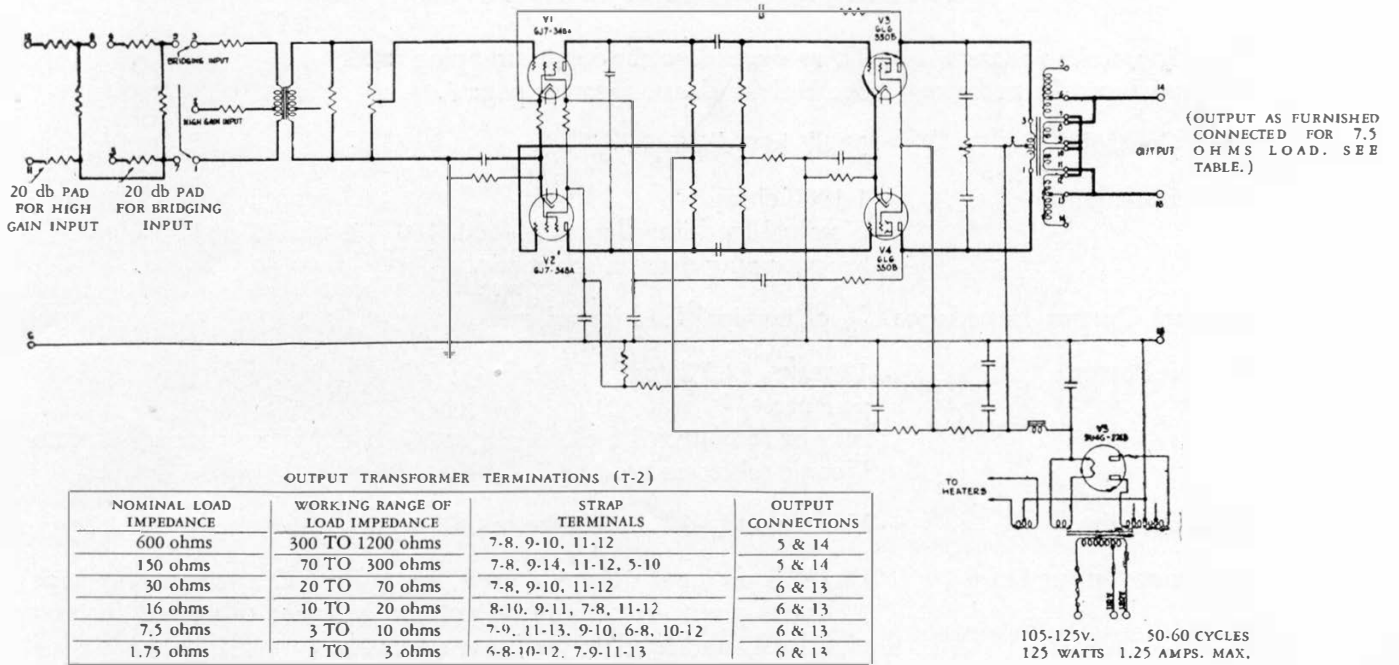
Schematic of 124E Amplifier
