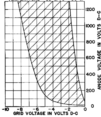
TYPICAL CONTROL CHARACTERISTICS, SHADED AREA SHOWS RANGE OF CHARACTERISTICS, CONDENSED MERCURY TEMPERATURE -55°C. TO +80°C.
