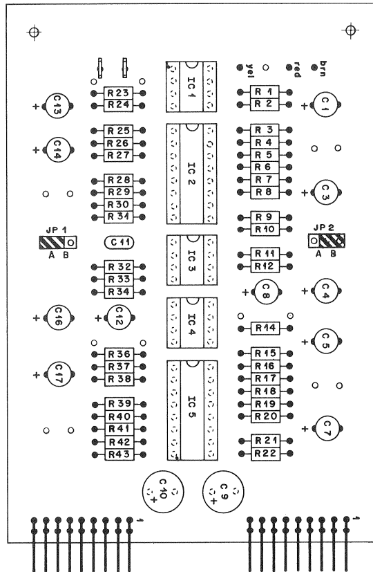
M/S OUTPUT AMPLIFIER WITH TEST GENERATOR 1.727.442.00 GRP45
