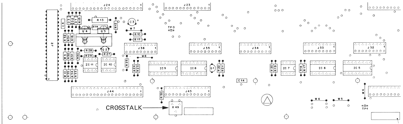
AUDIO CONTROL 1.727.40X.XX GRP40
