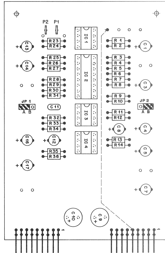
M/S OUTPUT AMPLIFIER PBO 1.727.452.00 GRP45
