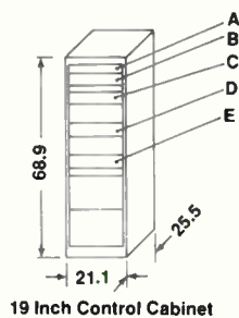
19 Inch Control Cabinet
