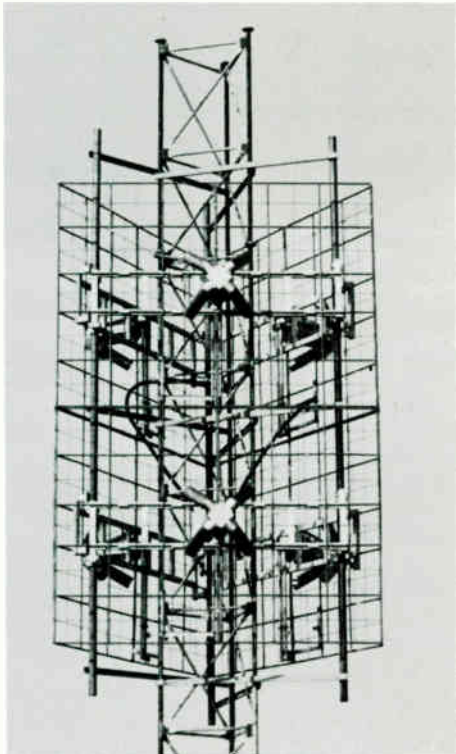
Above: G5CPS with Radome. Below: Type 1082 panel antenna.
