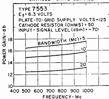
GAIN CHARACTERISTICS CATHODE-DRIVE SERVICE
