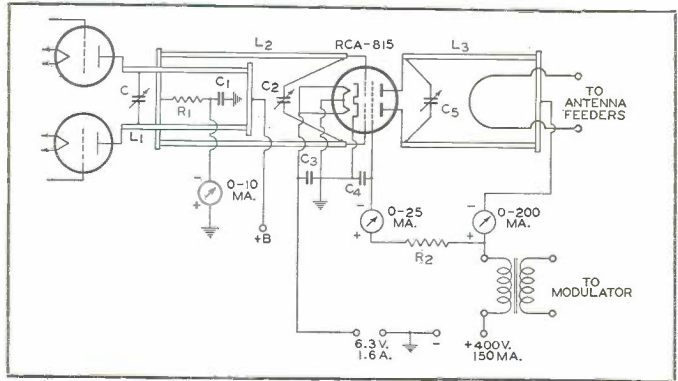
112-116-Mc PLATE-MODULATED R-F POWER AMPLIFIER Power Output 45 Watts (ICAS) *
