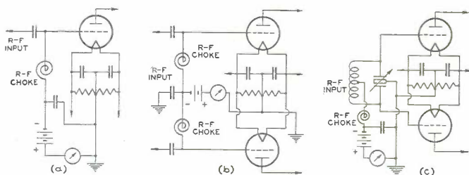
CONNECTIONS FOR FIXED BIAS SUPPLY
