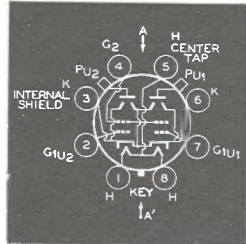
Bottom View of Socket Connections
