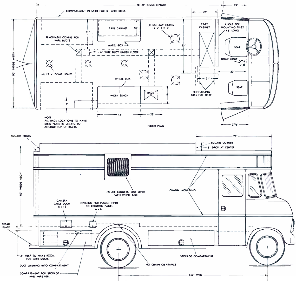
EFFICIENT SPACE UTILIZATION —Floor plan and elevation of a typical TJ-72 Mobile Unit showing provisions made for accommodating complete TV Tape Recording Equipment.
