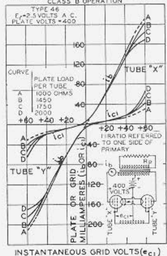
DYNAMIC TRANSFER CHARACTERISTICS CLASS B OPERATION
