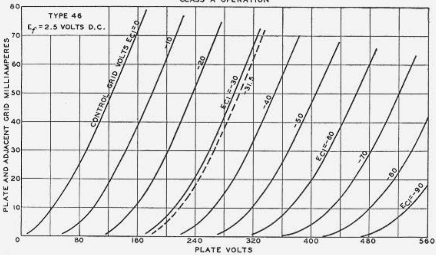
AVERAGE PLATE CHARACTERISTICS CLASS A OPERATION
