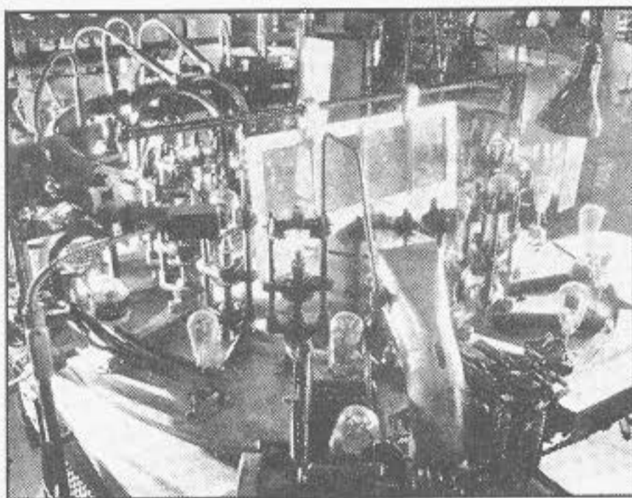
Bulb Sealing and Exhausting
