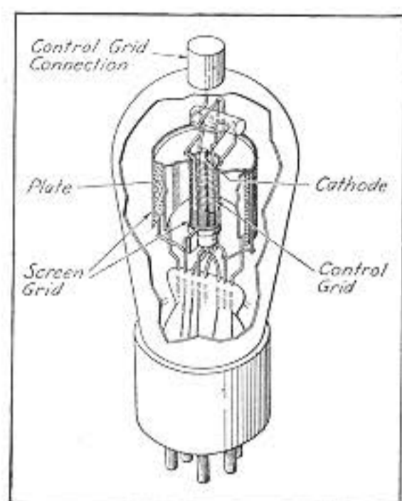
Interior View of '24-A
