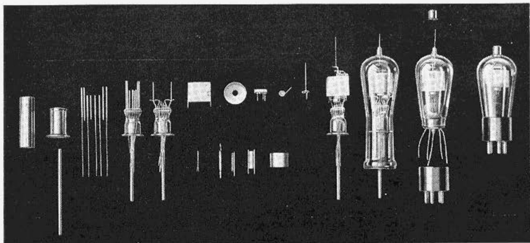
Parts Assembly of the '24-A
