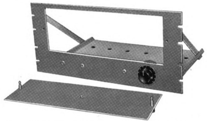
Type 36-B Panel and Shelf Assembly with Door Removed
