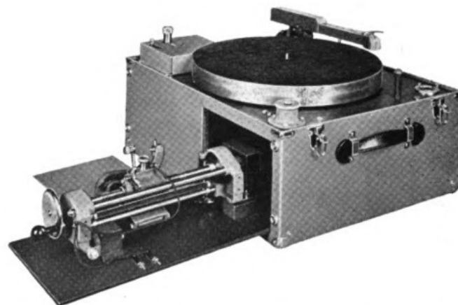
Showing method of Mounting Recording Attachment while transporting unit.
