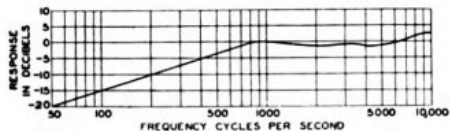
Typical frequency response of MI-11850-C and MI-4887 based upon optical measurements of the stylus tip motion for constant input
