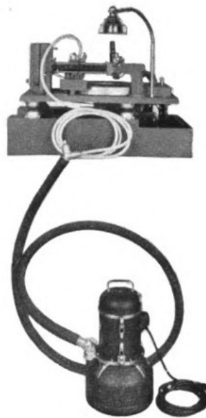
Recording Suction and Hose Equipment Attached to Type 73-A Recorder
