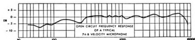
Frequency in Cycles per Second
