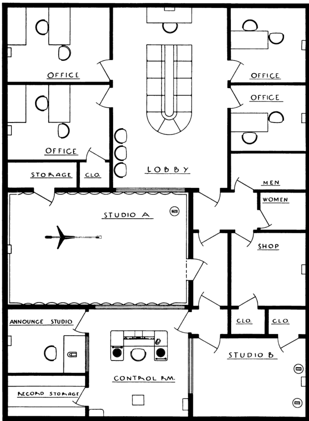
SUGGESTED BROADCAST STUDIO LAYOUT
