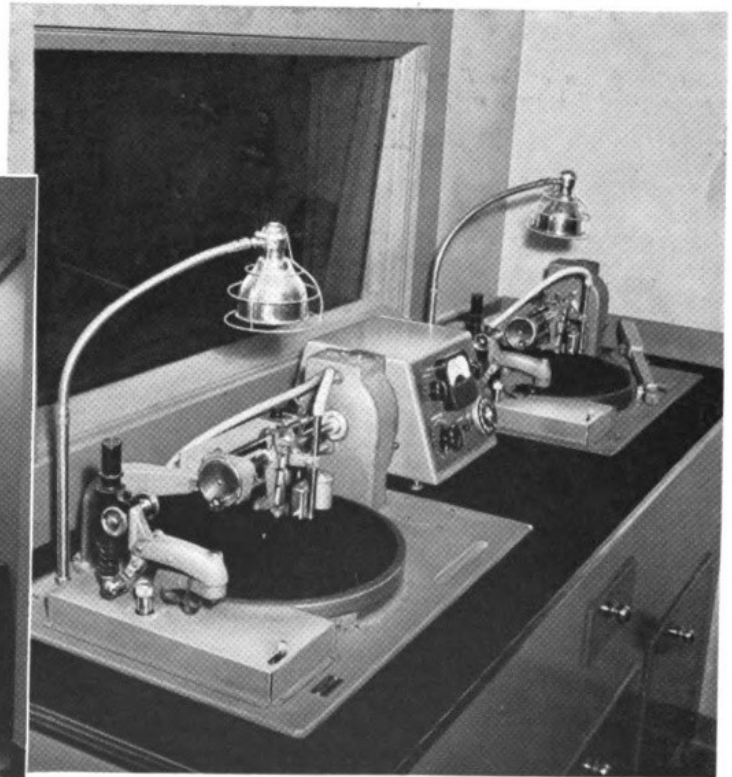
▲ Professional Recorder Installation at the studios of KGLO, Mason City, Iowa
