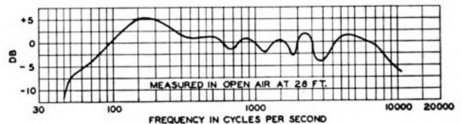
AVERAGED FREQUENCY RESPONSE OF TYPICAL 64-B LOUD SPEAKER
