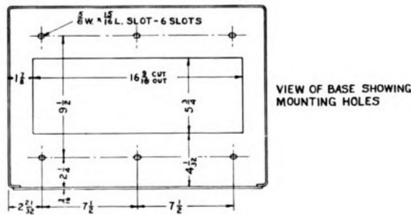
OUTLINE DIMENSIONS OF 9AX CABINET RACK
