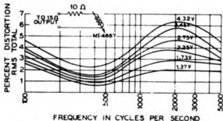
Typical distortion measurements for MI-11850-C and MI-4887 Recording Head
