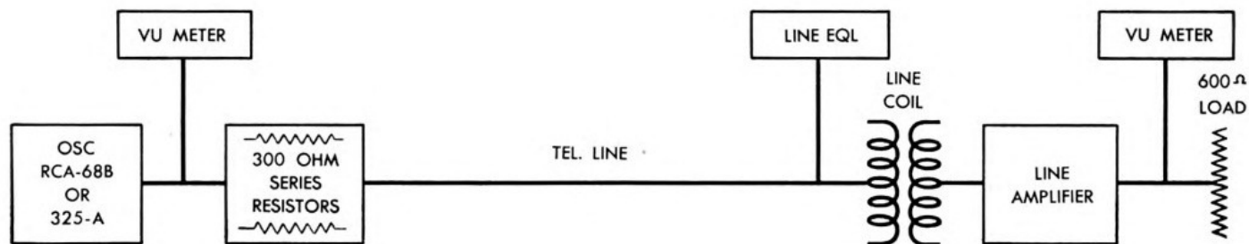
TYPICAL SET-UP FOR EQUALIZING TELEPHONE LINES
