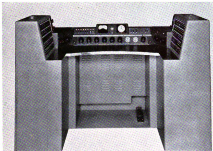
◀ Type 2-A Desk built for CBS with view directly below it showing front and side open.
