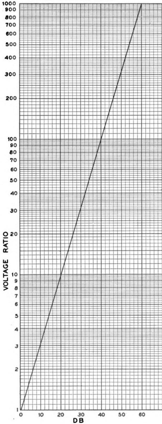
Voltage Ratio 1 DB
