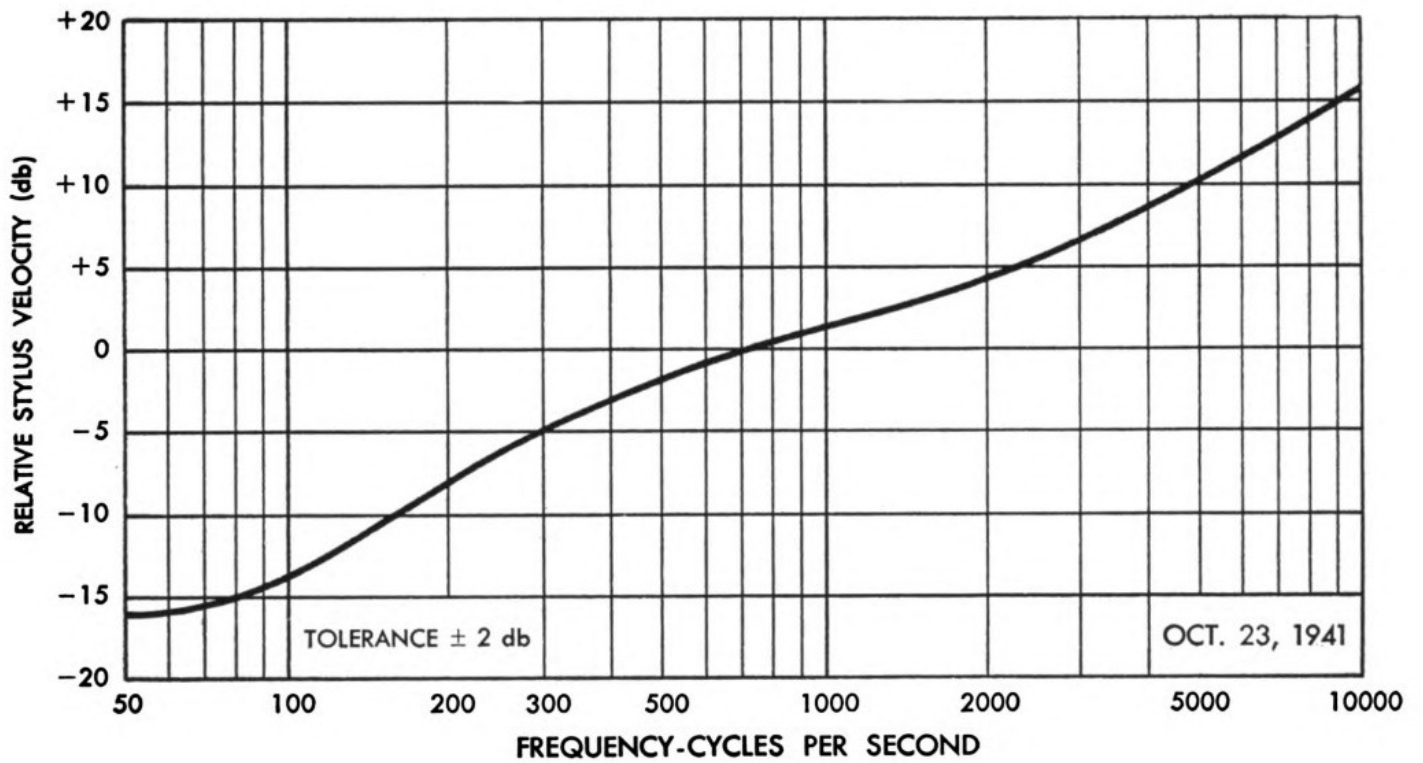
Reproducing characteristics for Lateral Transcriptions as set forth by the Recording and Reproducing Standards Committee of the National Association of Broadcasters.
