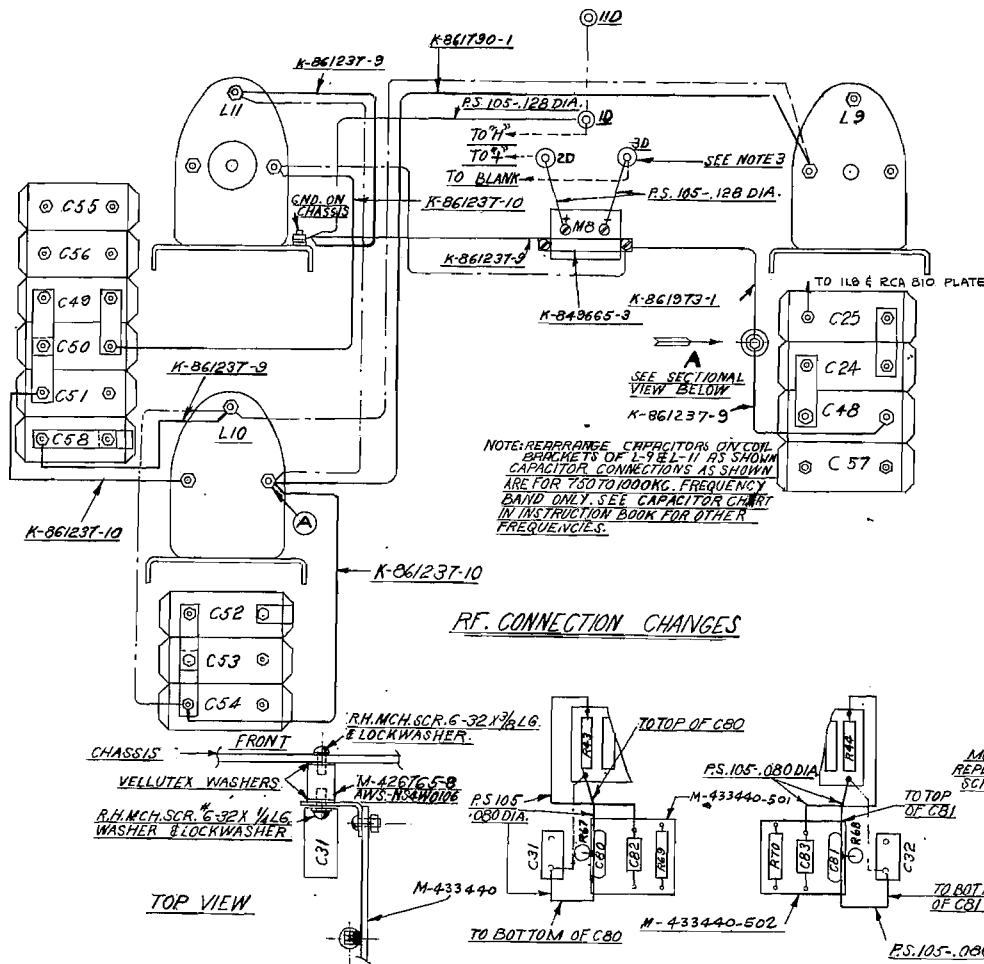
Figure 16—BT-A-250L Connection Changes (P-722508)
