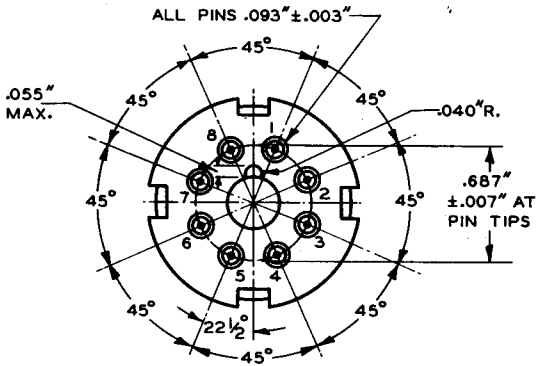
BOTTOM VIEW OF BASE
