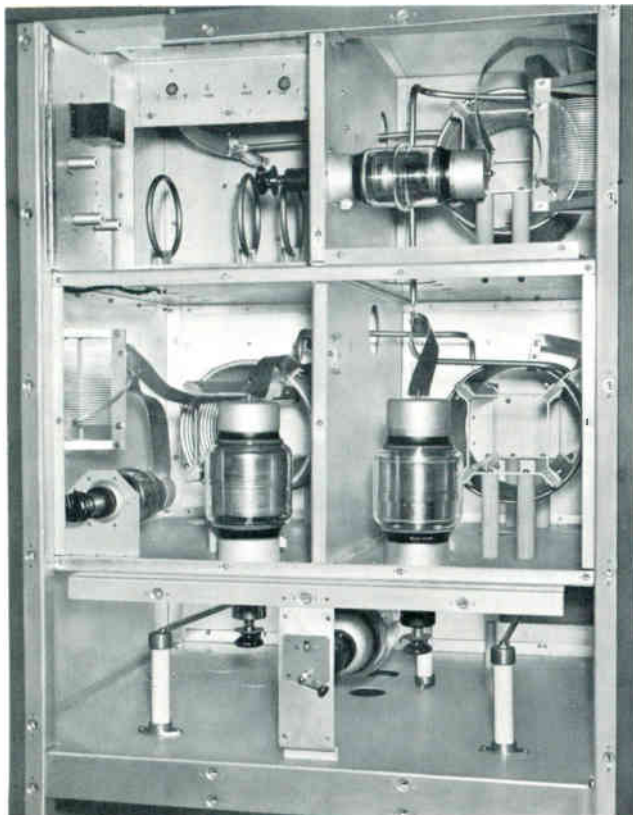
Upper rear of exciter portion of the BTA-50H1 showing the combining and output networks.
