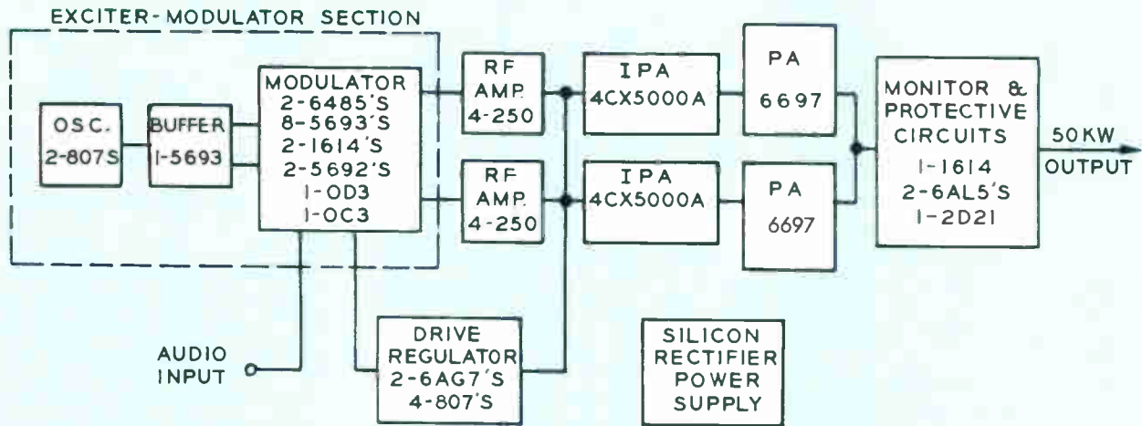
Simplified block diagram of the BTA-50H.
