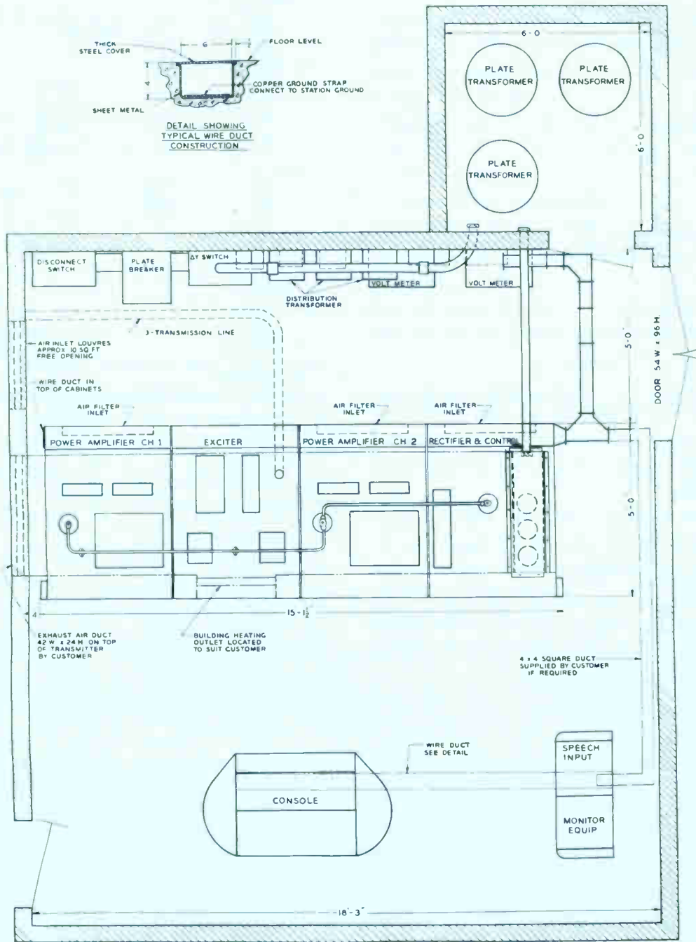
Typical floor plan for the BTA-50H1 Transmitter.
