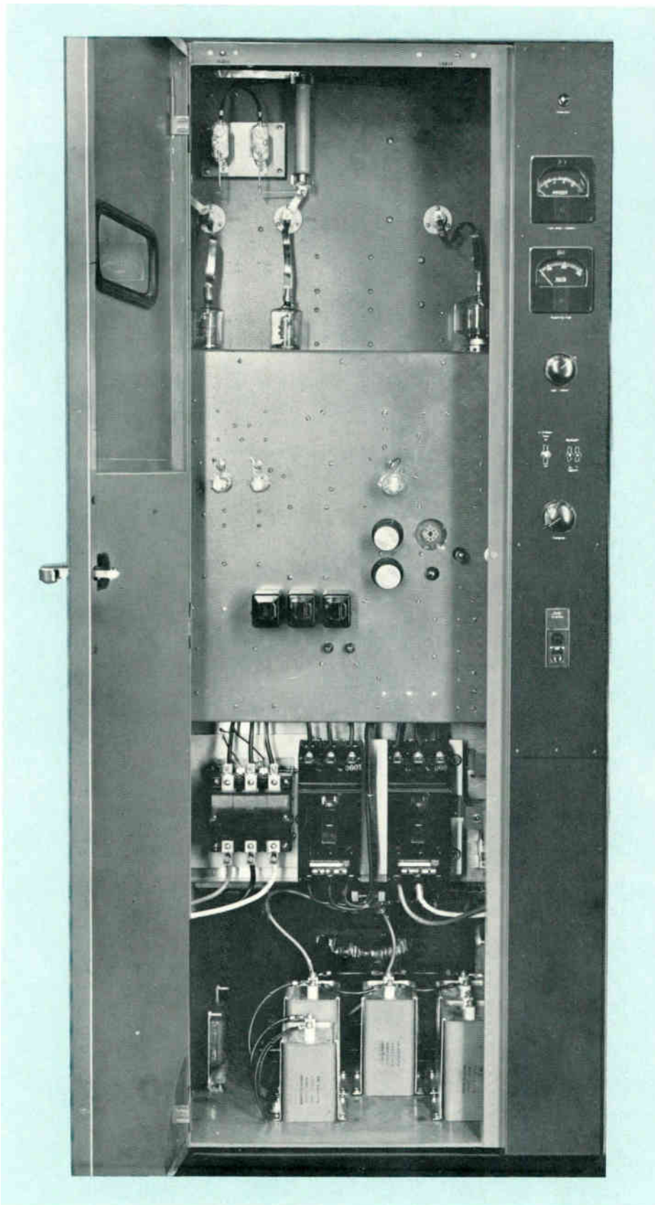
Driver cabinet including exciter and control panel.
