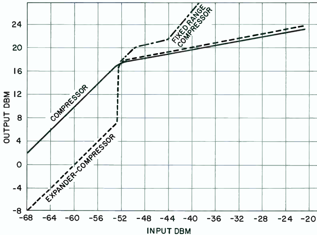
Transfer characteristics of BA-28A Program Amplifier.
