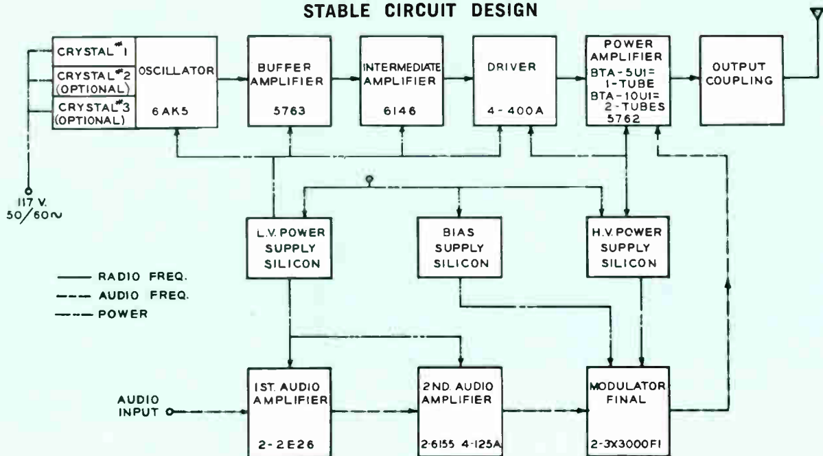
Block diagram of Type BTA-5U1 and BTA-10U1 Transmitters.
