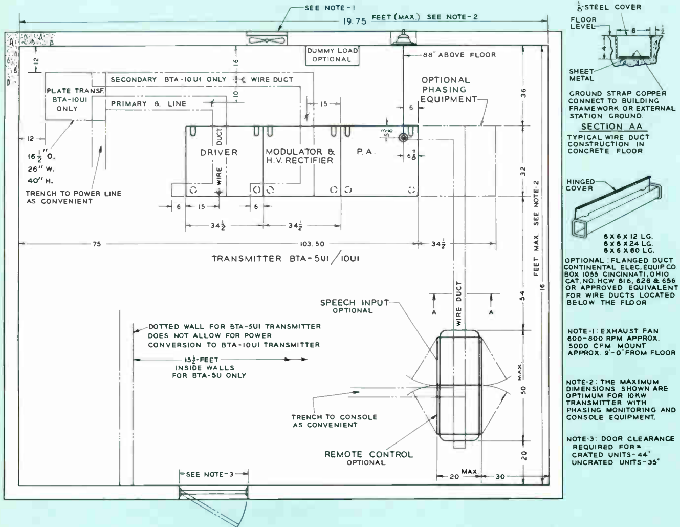
Typical floor plan for BTA-5U1 and BTA-10U1 transmitters. External plate transformers are required only for the BTA-10U1 transmitter since the transformer for the BTA-5U1 can be mounted in the PA cabinet.
