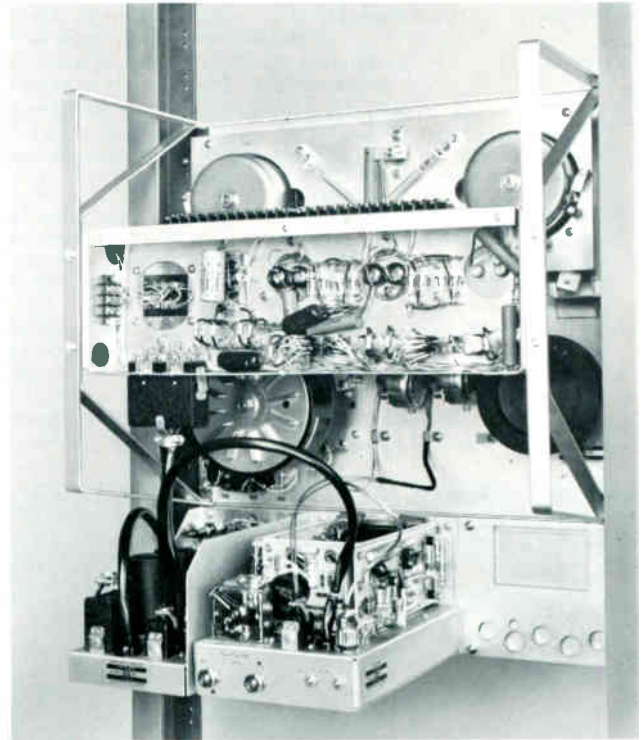
Front and rear views of RT-21B Tape Recorder showing tape transport at top, and control panel below. In rear view the modular control unit is shown at left and amplifier module in center. Space at right supports a second amplifier module for stereo tape operation.
