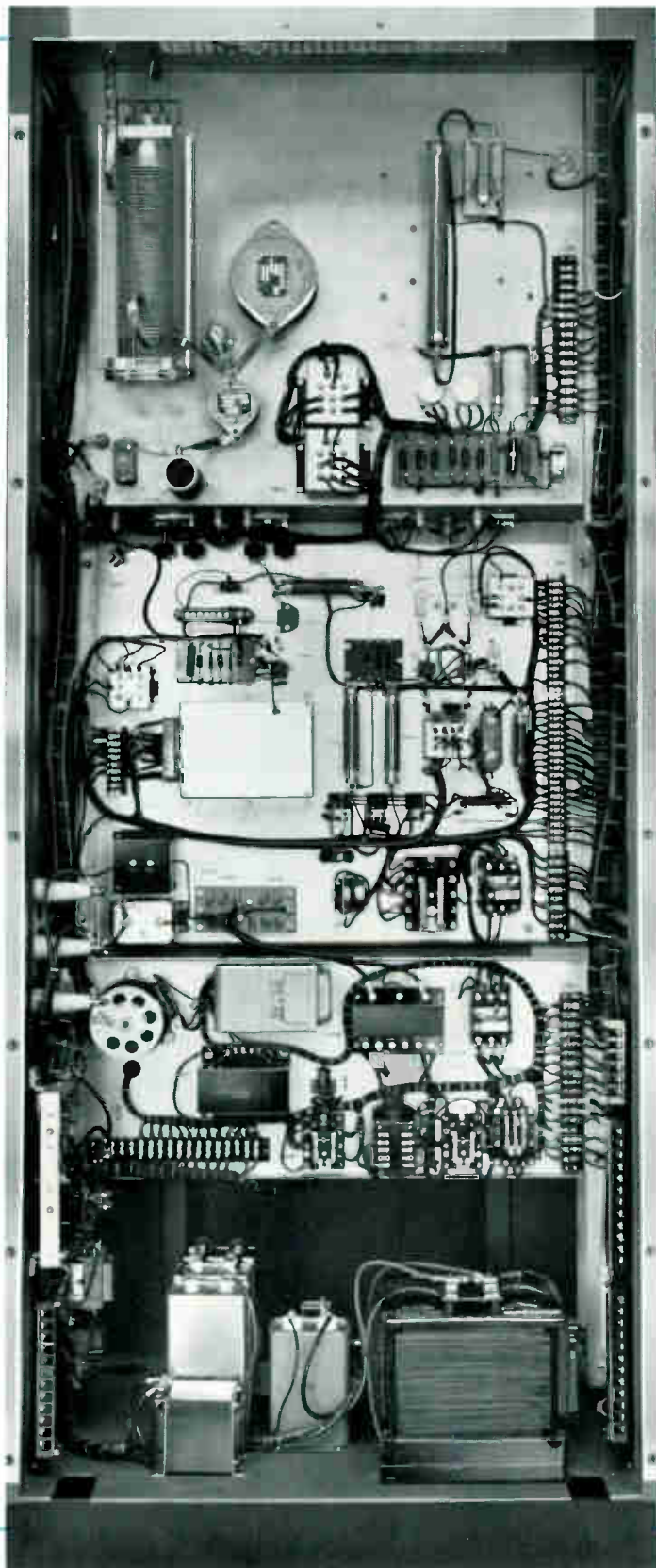
Rear of the BTA-5T1 exciter-driver cabinet.
