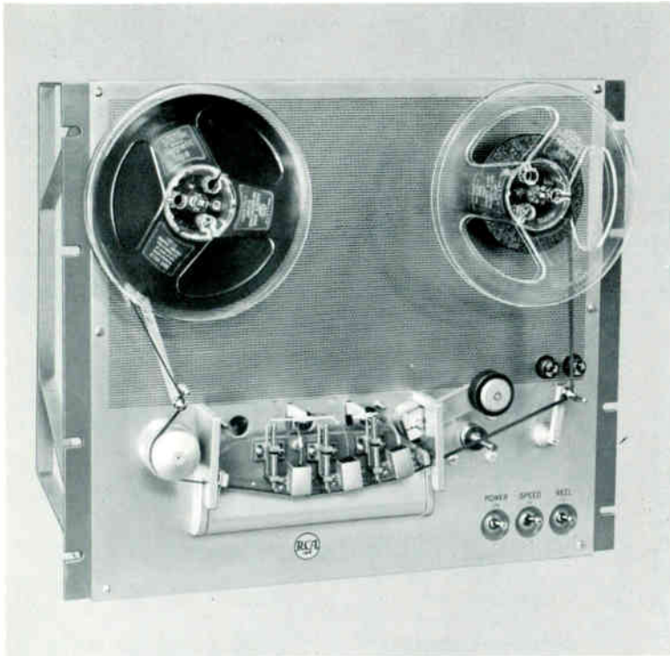
RT-21B Tape Transport with cover removed to reveal magnetic heads. Note cut-out provision on left for optional fourth head kit for playing pre-recorded stereo tapes.
