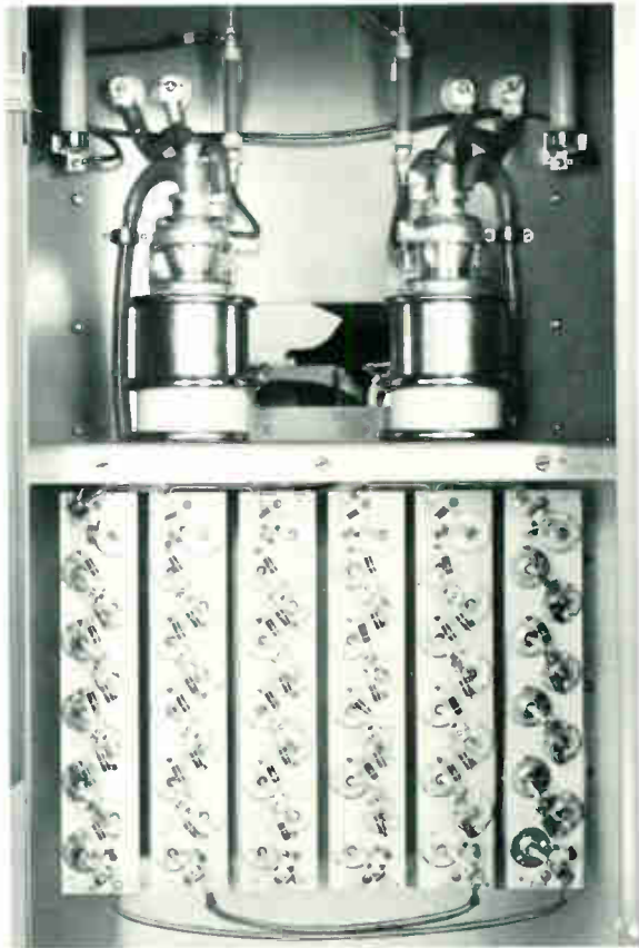
Modulator tubes and silicon high voltage rectifiers with cover removed.
