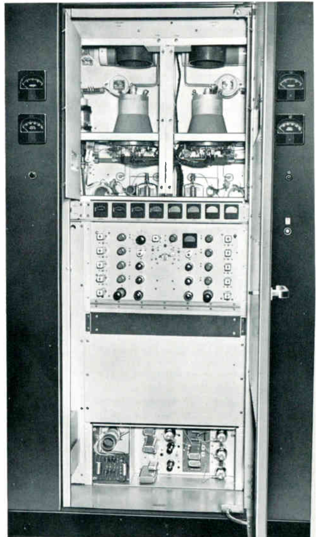
Front section of the exciter-modulator containing all components from oscillator through the driver stages.
