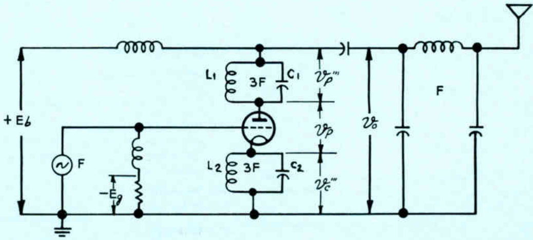
Simplified schematic of the new high efficiency PA stage. The adjustment of the circuit differs from a conventional class "C" only in that the coils L_1 and L_2 are resonated for maximum efficiency.
