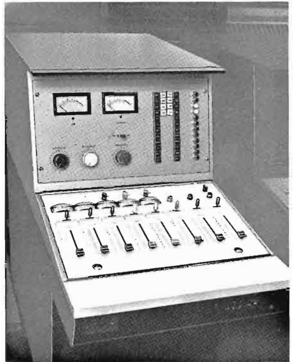
Three console housings designed for in-line installation will offer Station KRON complete studio audio facilities. Shown at left is eight-channel microphone mixer with three sub-mixing channels. Up to six microphones per channel can be selected. Note the vertical type faders, convenient bus selectors, and reverberation and equalizer controls. The second section is an eight-channel master mixer featuring latest RCA remote AGC meters and BA-40 series amplifiers.
