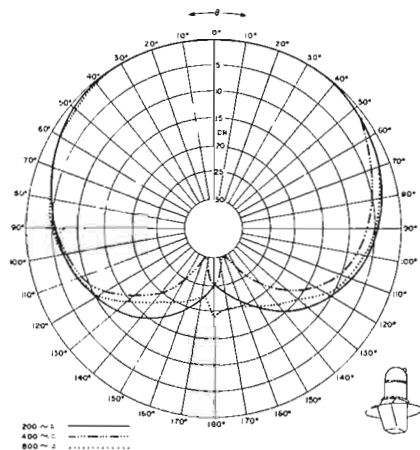
Horizontal Pattern of MI-10001-C Microphone.
