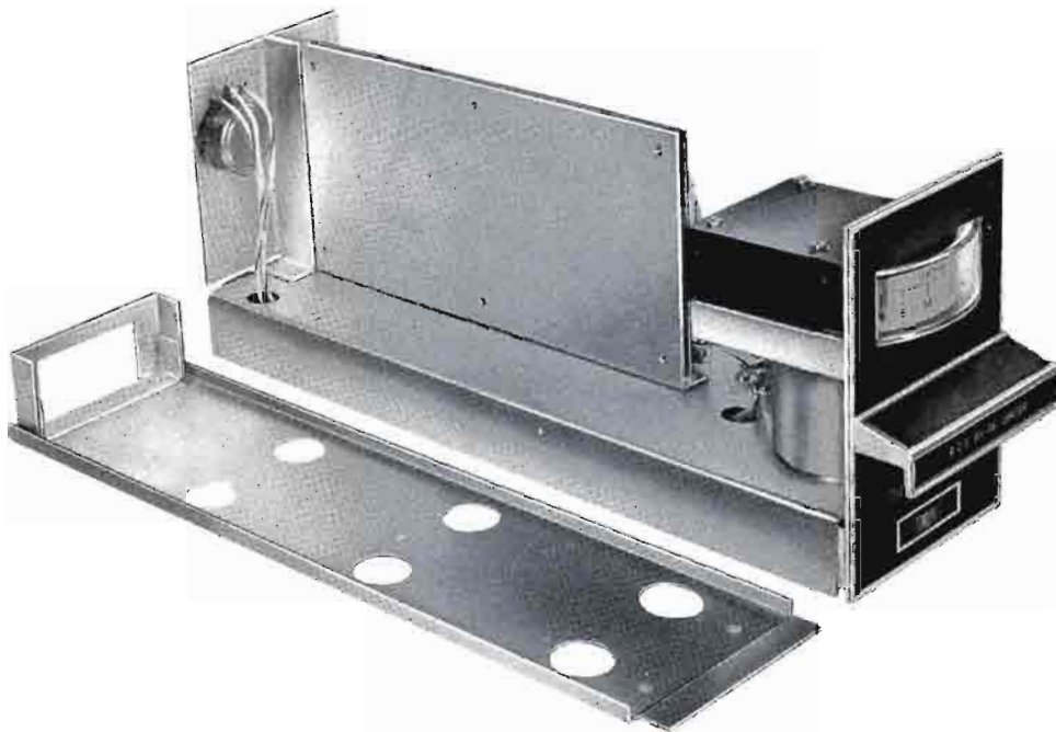
The BA-46 Limiter Amplifier, MI-11456 shown with the guide assembly ready for mounting in the BR-22 Mounting Shelf. The amplifier prevents over-modulation of the system on heavy passages of music or speech.
