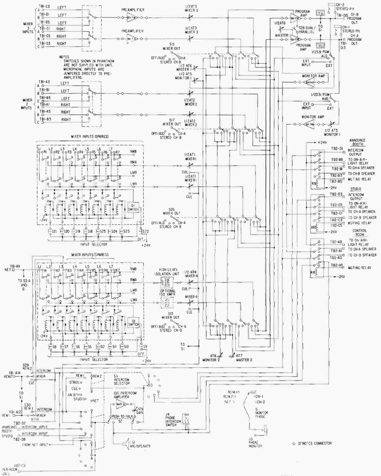
Functional Diagram
