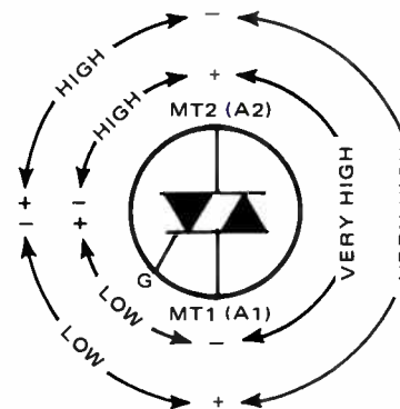
TRIAC
