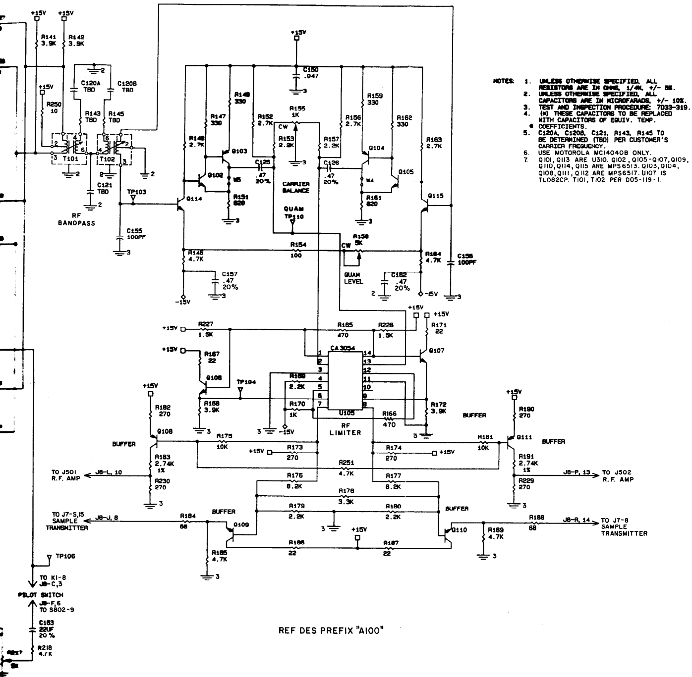
FIGURE 8-9 SCHEMATIC DIAGRAM ENCODER ASSEMBLY
