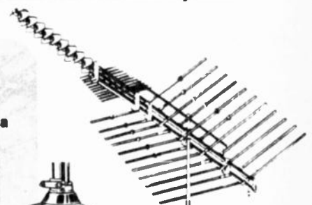
"ULTRA-FRINGER" ANTENNA 18-02172WX
