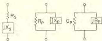
Figure 4. Series and parallel components of impedance.
