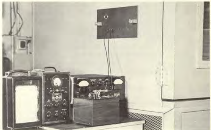
Long leads from capacitor in conditioning chamber, as shown here, have a negligible effect on measurement accuracy. Bridge output can also operate a recorder to give a continuous record of environmental tests.
