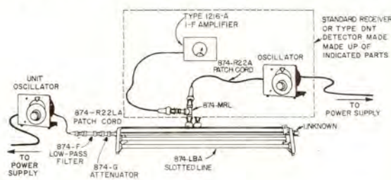
Typical measurement setups showing use of slotted line, VSWR indicator (left), and heterodyne detector (right).
