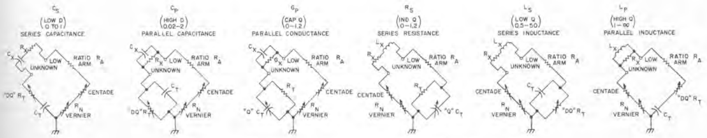
Elementary schematics of the capacitance, conductance, resistance, and reactance bridges.
