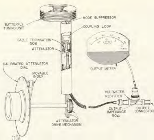
Functional diagram of output system.
