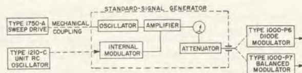
Figure 2. Modulation methods.
