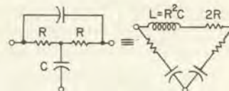
Figure 4. Equivalent wye and delta networks for a resistor with capacitance to shield.
