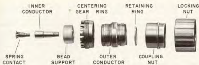
Type 900-BT Precision Coaxial Connector.
