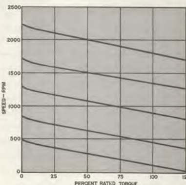
Speed-torque characteristics of a typical motor and speed control installation.
