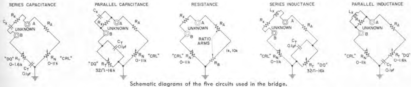
Schematic diagrams of the five circuits used in the bridge.
