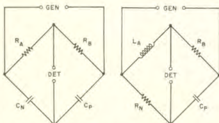
Figure 2. Circuits for capacitance bridges in which like reactances, C_N and C_P , or unlike reactances, L_A and C_P , are compared.
