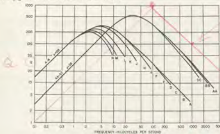
Figure 1. Q versus frequency for typical units.
