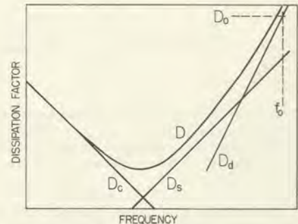
Figure 2. Dissipation factor variation with frequency showing the relative contributions of the several loss components for air-core inductors.
