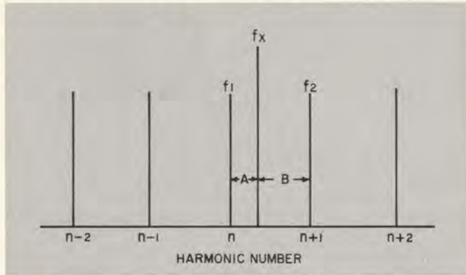
Figure 2. Relation between an unknown frequency and a series of standard-frequency harmonics.
