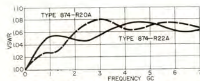
Average VSWR of Types 874-R20A and -R22A.
