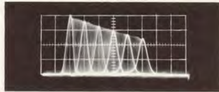
Oscilloscope showing pulse shape and amplitude as delay setting is varied. Tektronix 541 Oscilloscope, 53K/54K Pre-Amplifiers; sweep, 0.1 \mu sec/cm.
