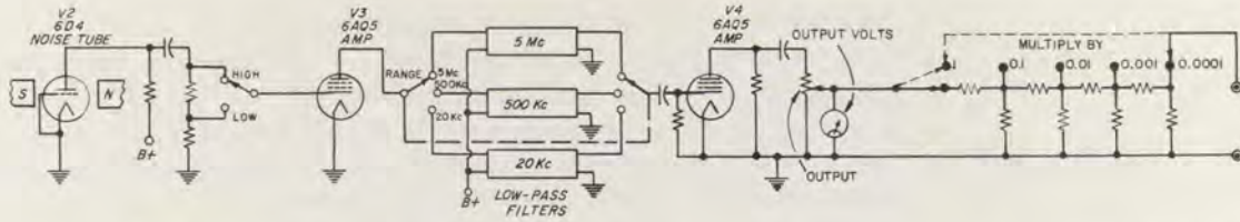
Elementary schematic of the generator.
