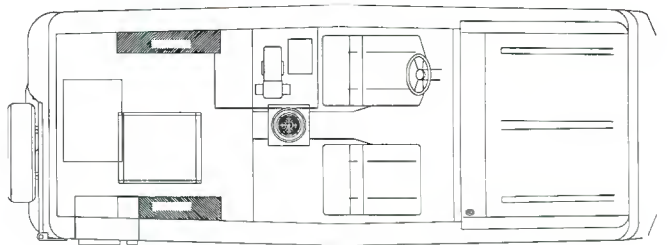
M-11ENG Floor Plan
