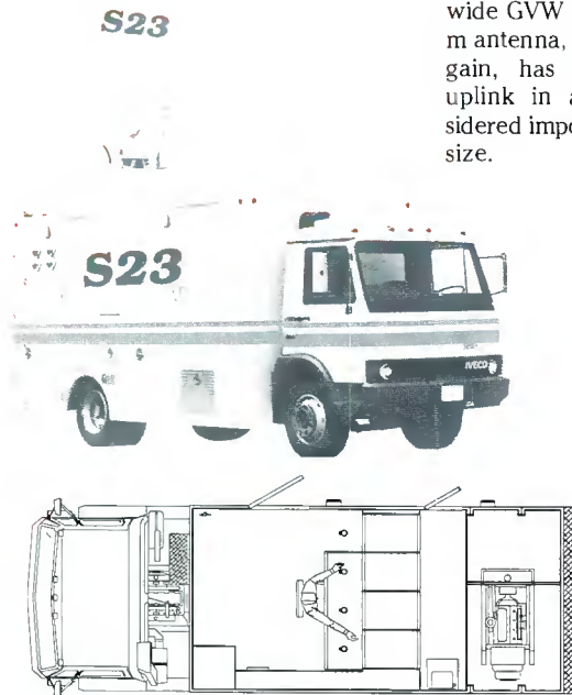
S-23 Floor Plan
