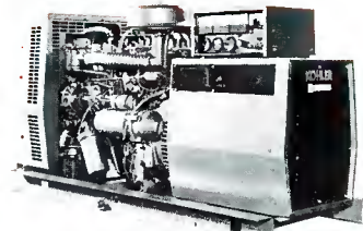
22.5 KW Gasoline
