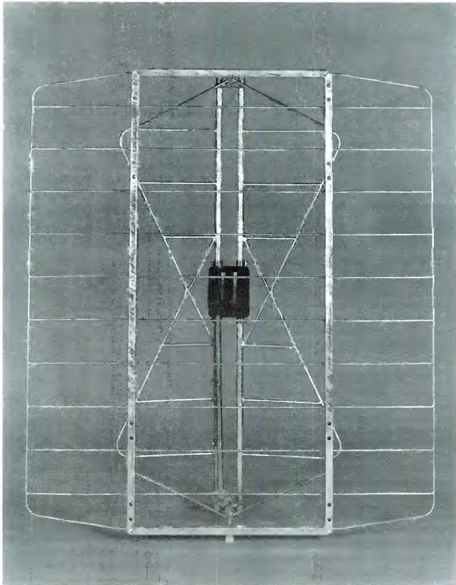
VHF DELTAWING
