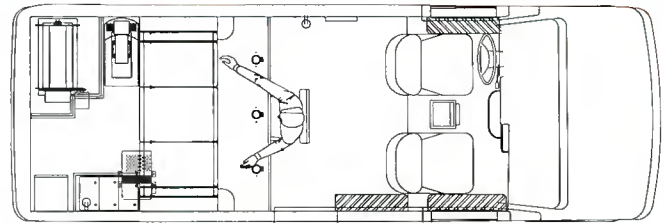
M-1 Floor Plan
